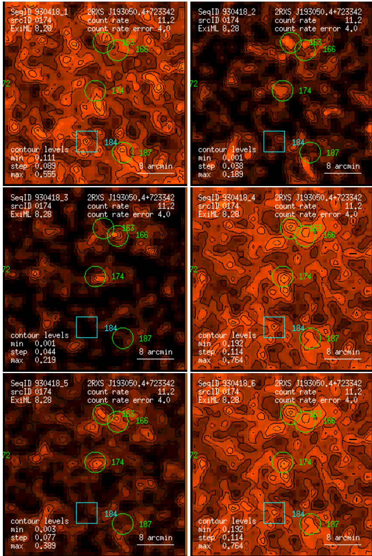
Figure 174: RASS 930418: detection 0174: band rate images, Gaussian filter: (1) PSPC channels 11 – 41, (2) 52 – 90, (3) 91 – 201, (4) 11 – 235, (5) 52 – 201, (6) 11 – 201. Broad band rates in counts/ks. Band rate contour levels in counts/ks/arcmin 2 .
