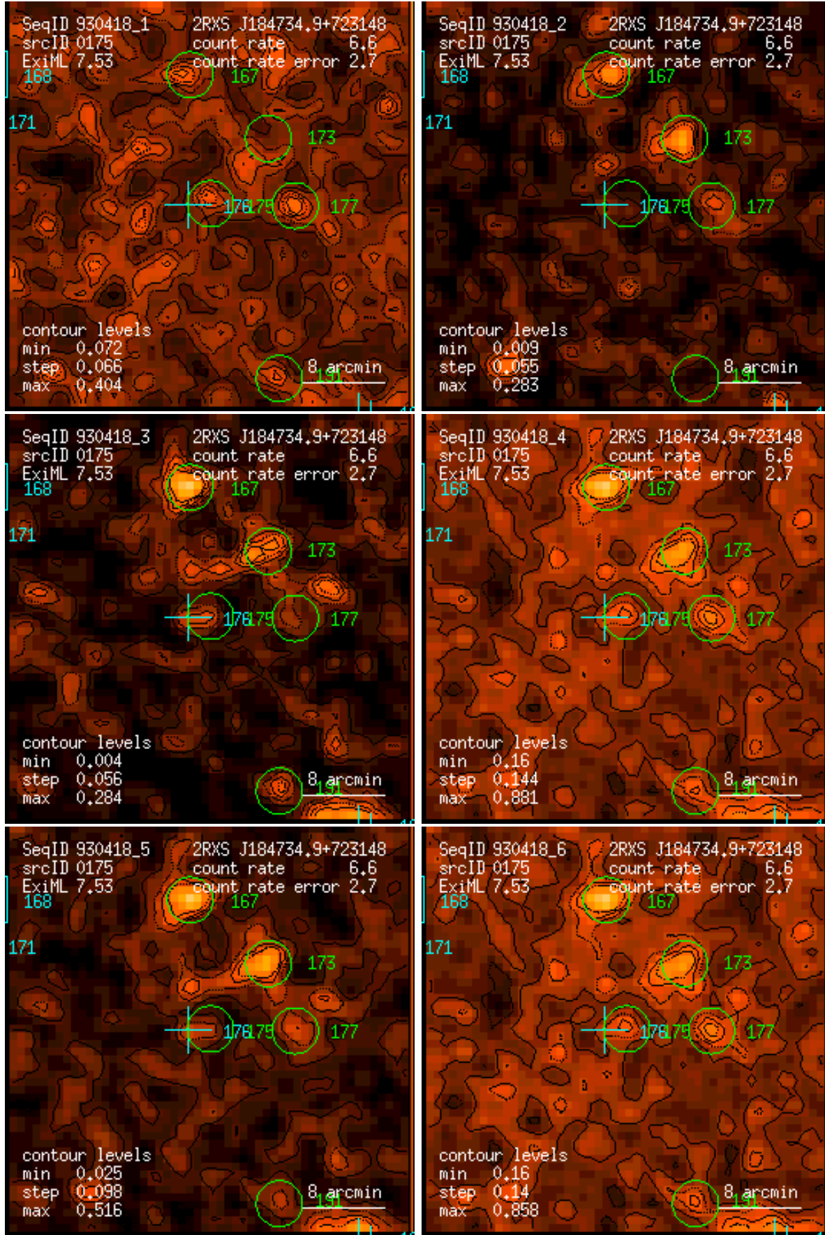
Figure 175: RASS 930418: detection 0175: band rate images, Gaussian filter: (1) PSPC channels 11 – 41, (2) 52 – 90, (3) 91 – 201, (4) 11 – 235, (5) 52 – 201, (6) 11 – 201. Broad band rates in counts/ks. Band rate contour levels in counts/ks/arcmin 2 .
