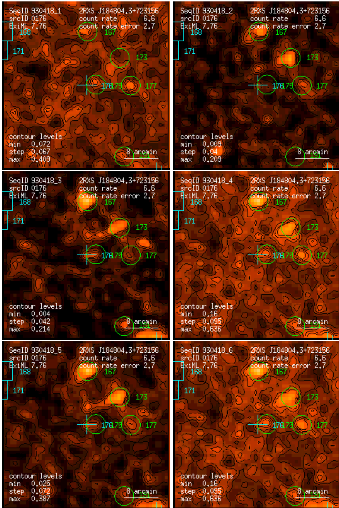
Figure 176: RASS 930418: detection 0176: band rate images, Gaussian filter: (1) PSPC channels 11 – 41, (2) 52 – 90, (3) 91 – 201, (4) 11 – 235, (5) 52 – 201, (6) 11 – 201. Broad band rates in counts/ks. Band rate contour levels in counts/ks/arcmin 2 .
