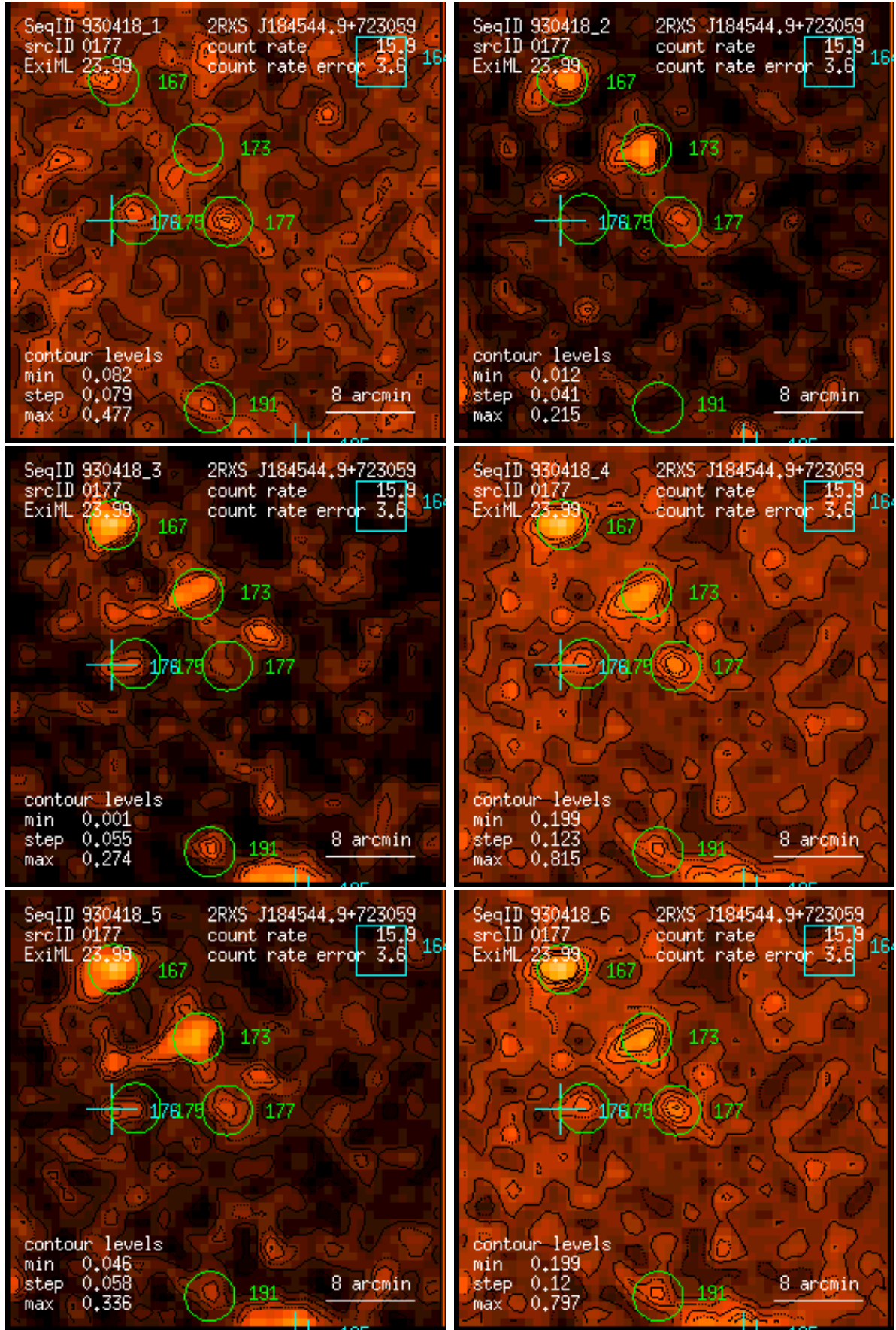
Figure 177: RASS 930418: detection 0177: band rate images, Gaussian filter: (1) PSPC channels 11 – 41, (2) 52 – 90, (3) 91 – 201, (4) 11 – 235, (5) 52 – 201, (6) 11 – 201. Broad band rates in counts/ks. Band rate contour levels in counts/ks/arcmin 2 .
