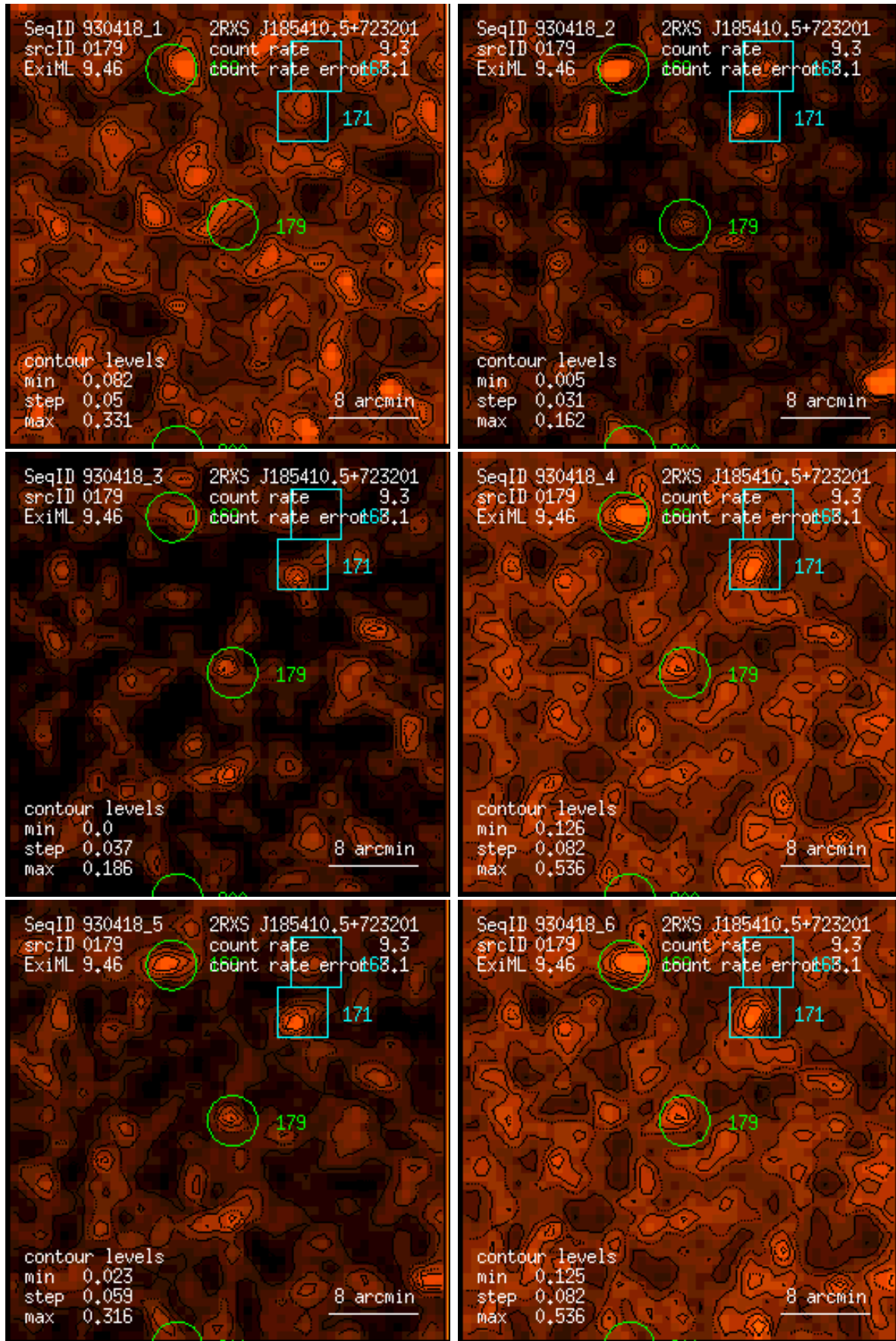
Figure 179: RASS 930418: detection 0179: band rate images, Gaussian filter: (1) PSPC channels 11 – 41, (2) 52 – 90, (3) 91 – 201, (4) 11 – 235, (5) 52 – 201, (6) 11 – 201. Broad band rates in counts/ks. Band rate contour levels in counts/ks/arcmin 2 .
