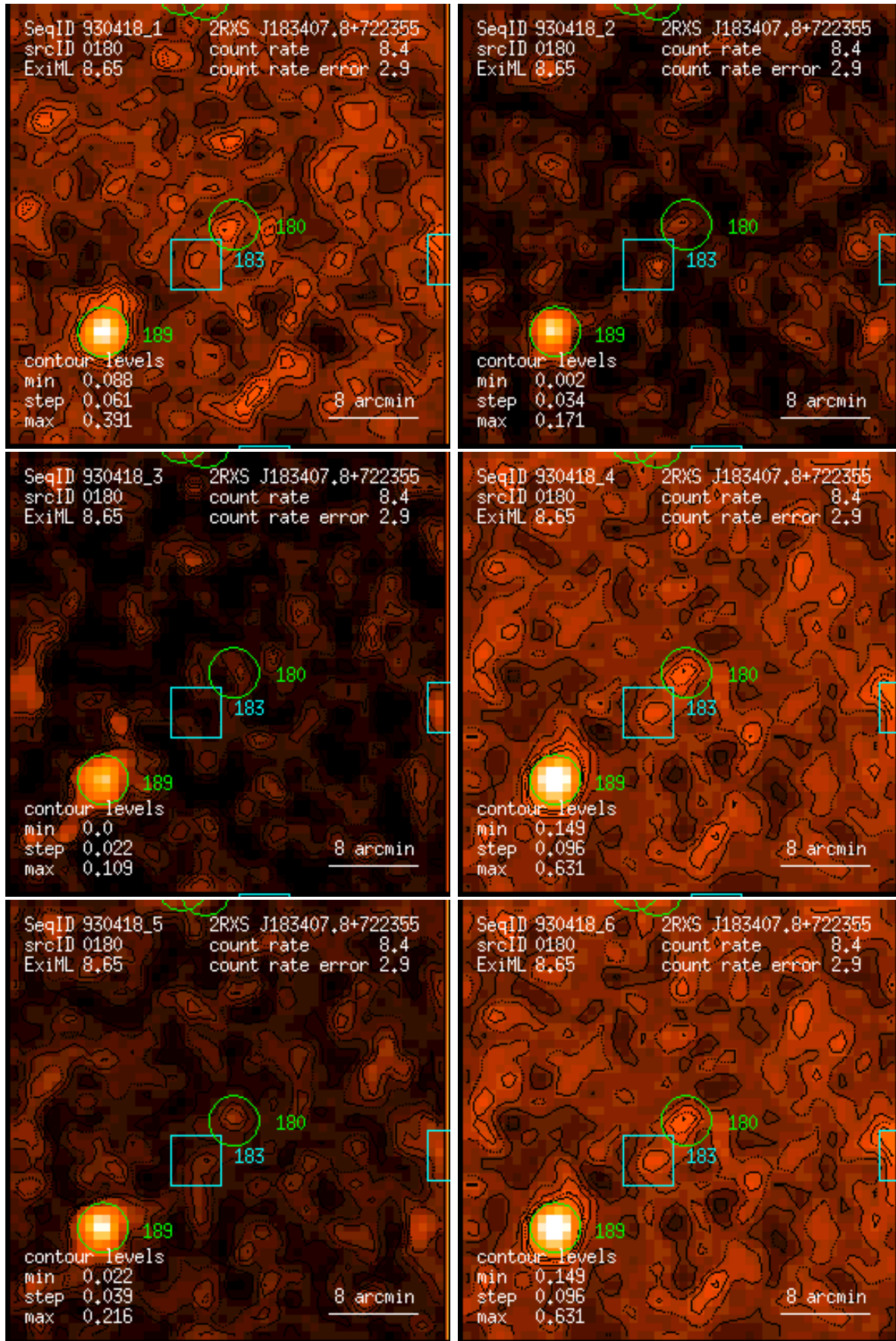
Figure 180: RASS 930418: detection 0180: band rate images, Gaussian filter: (1) PSPC channels 11 – 41, (2) 52 – 90, (3) 91 – 201, (4) 11 – 235, (5) 52 – 201, (6) 11 – 201. Broad band rates in counts/ks. Band rate contour levels in counts/ks/arcmin 2 .
