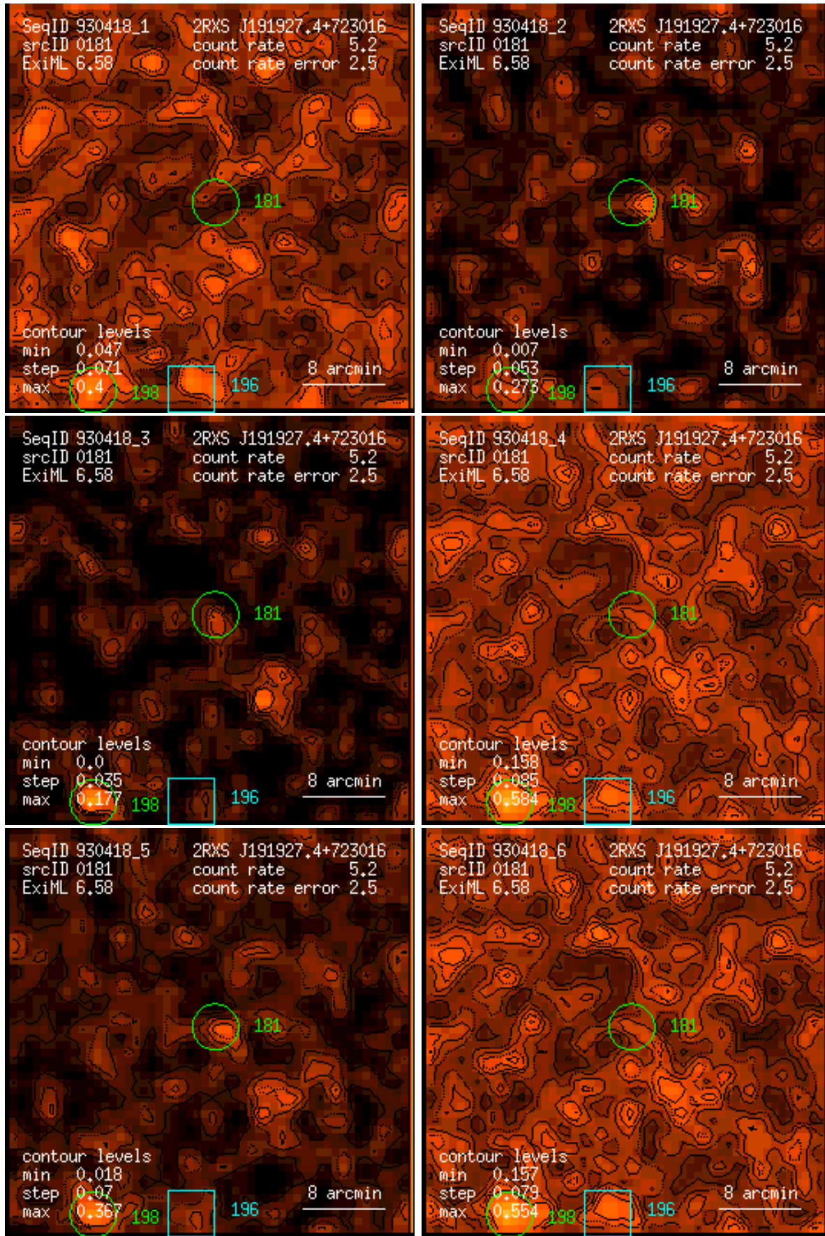
Figure 181: RASS 930418: detection 0181: band rate images, Gaussian filter: (1) PSPC channels 11 – 41, (2) 52 – 90, (3) 91 – 201, (4) 11 – 235, (5) 52 – 201, (6) 11 – 201. Broad band rates in counts/ks. Band rate contour levels in counts/ks/arcmin 2 .
