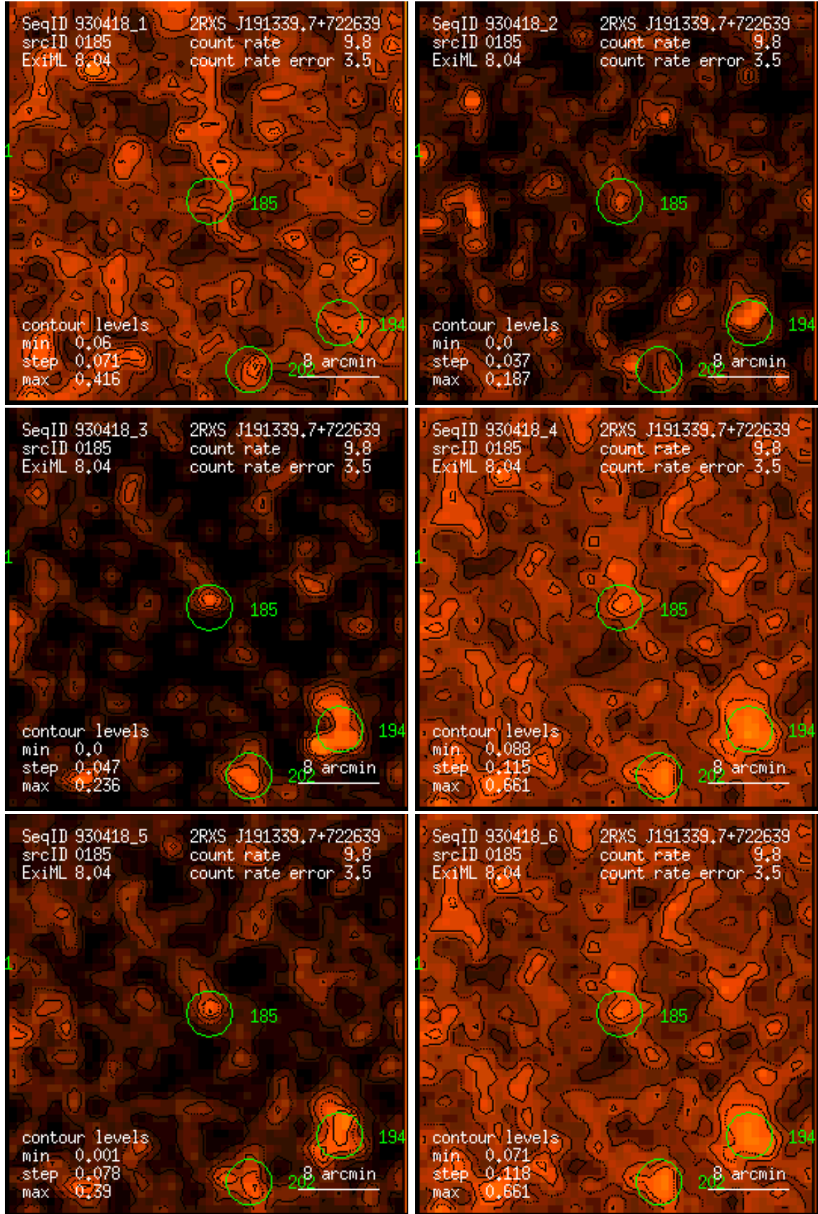
Figure 185: RASS 930418: detection 0185: band rate images, Gaussian filter: (1) PSPC channels 11 – 41, (2) 52 – 90, (3) 91 – 201, (4) 11 – 235, (5) 52 – 201, (6) 11 – 201. Broad band rates in counts/ks. Band rate contour levels in counts/ks/arcmin 2 .
