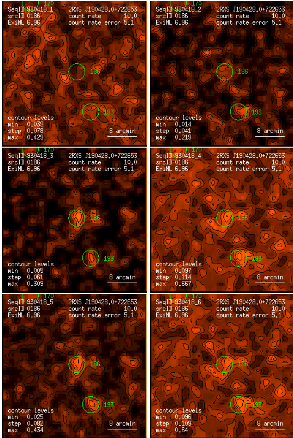
Figure 186: RASS 930418: detection 0186: band rate images, Gaussian filter: (1) PSPC channels 11 – 41, (2) 52 – 90, (3) 91 – 201, (4) 11 – 235, (5) 52 – 201, (6) 11 – 201. Broad band rates in counts/ks. Band rate contour levels in counts/ks/arcmin 2 .
