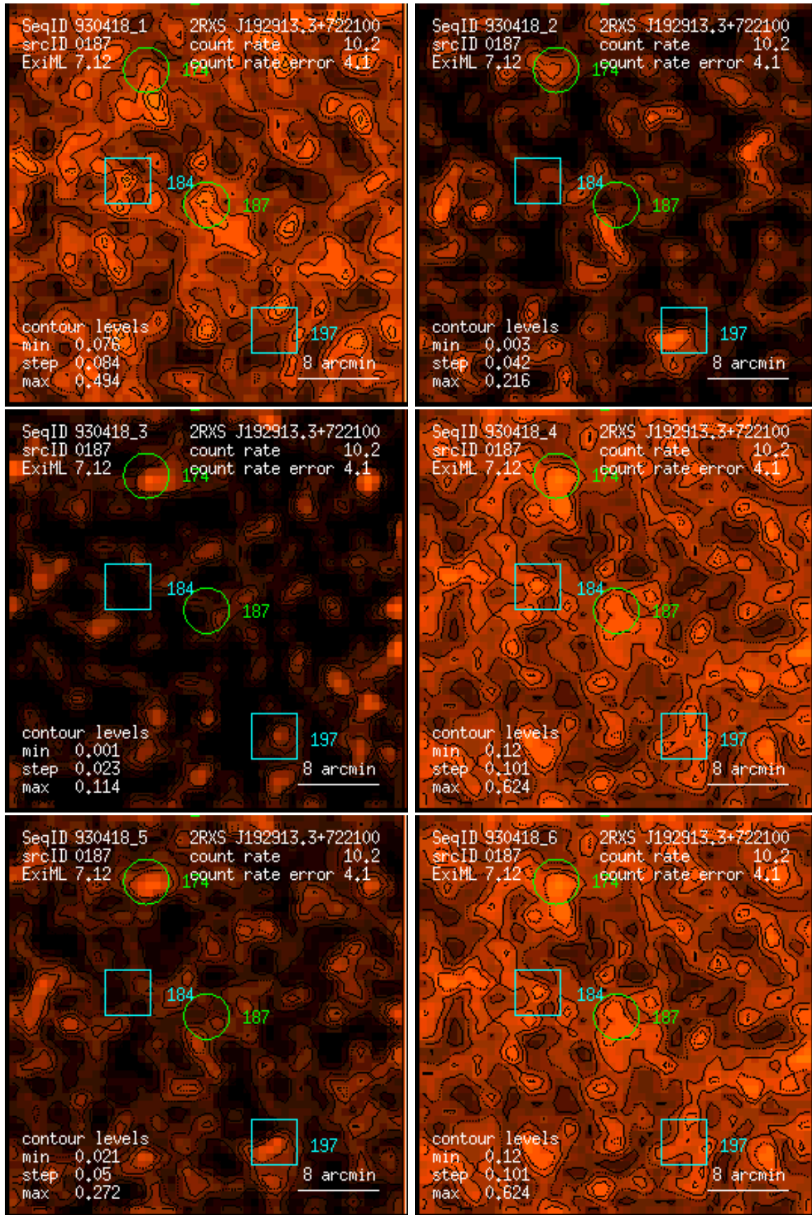
Figure 187: RASS 930418: detection 0187: band rate images, Gaussian filter: (1) PSPC channels 11 – 41, (2) 52 – 90, (3) 91 – 201, (4) 11 – 235, (5) 52 – 201, (6) 11 – 201. Broad band rates in counts/ks. Band rate contour levels in counts/ks/arcmin 2 .
