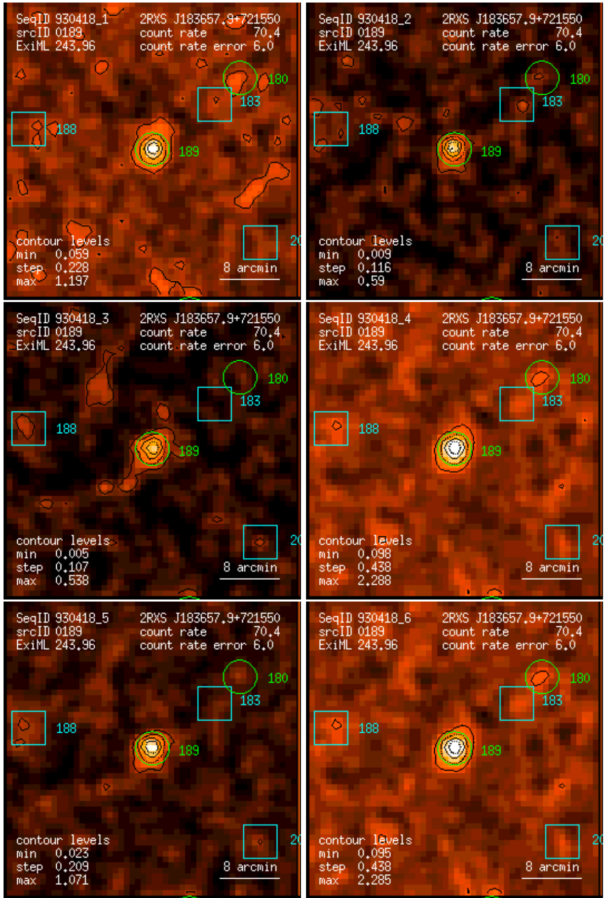
Figure 189: RASS 930418: detection 0189: band rate images, Gaussian filter: (1) PSPC channels 11 – 41, (2) 52 – 90, (3) 91 – 201, (4) 11 – 235, (5) 52 – 201, (6) 11 – 201. Broad band rates in counts/ks. Band rate contour levels in counts/ks/arcmin 2 .
