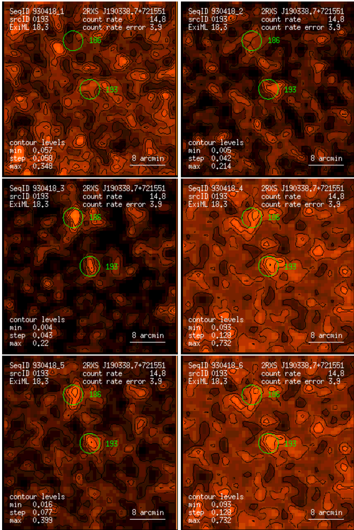
Figure 193: RASS 930418: detection 0193: band rate images, Gaussian filter: (1) PSPC channels 11 – 41, (2) 52 – 90, (3) 91 – 201, (4) 11 – 235, (5) 52 – 201, (6) 11 – 201. Broad band rates in counts/ks. Band rate contour levels in counts/ks/arcmin 2 .
