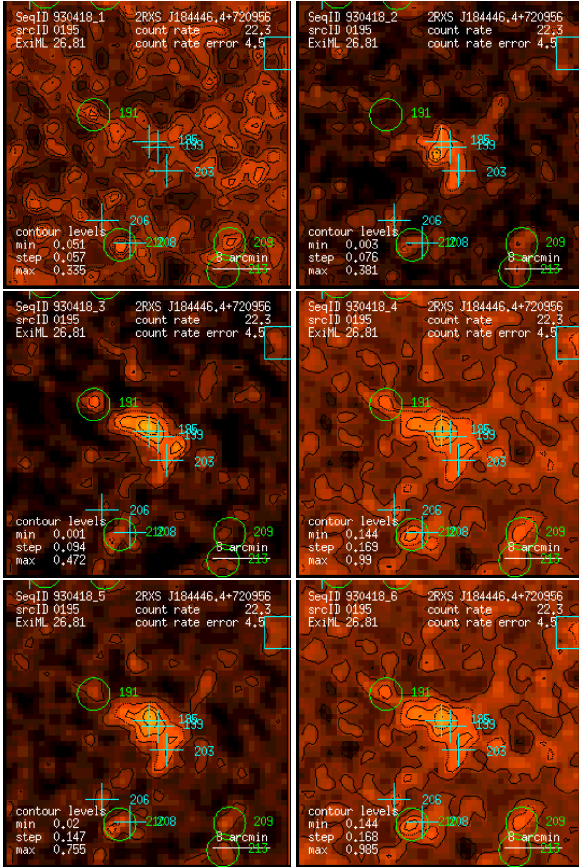
Figure 195: RASS 930418: detection 0195: band rate images, Gaussian filter: (1) PSPC channels 11 – 41, (2) 52 – 90, (3) 91 – 201, (4) 11 – 235, (5) 52 – 201, (6) 11 – 201. Broad band rates in counts/ks. Band rate contour levels in counts/ks/arcmin 2 .
