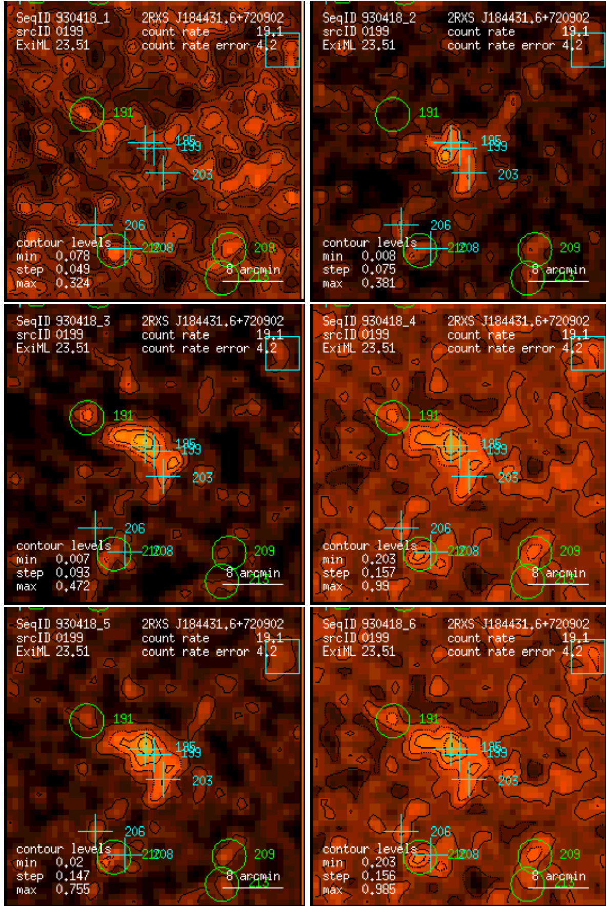
Figure 199: RASS 930418: detection 0199: band rate images, Gaussian filter: (1) PSPC channels 11 – 41, (2) 52 – 90, (3) 91 – 201, (4) 11 – 235, (5) 52 – 201, (6) 11 – 201. Broad band rates in counts/ks. Band rate contour levels in counts/ks/arcmin 2 .
