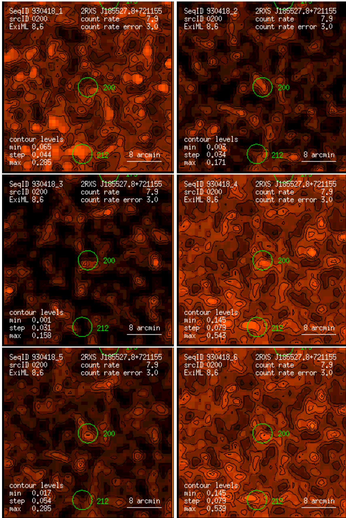
Figure 200: RASS 930418: detection 0200: band rate images, Gaussian filter: (1) PSPC channels 11 – 41, (2) 52 – 90, (3) 91 – 201, (4) 11 – 235, (5) 52 – 201, (6) 11 – 201. Broad band rates in counts/ks. Band rate contour levels in counts/ks/arcmin 2 .
