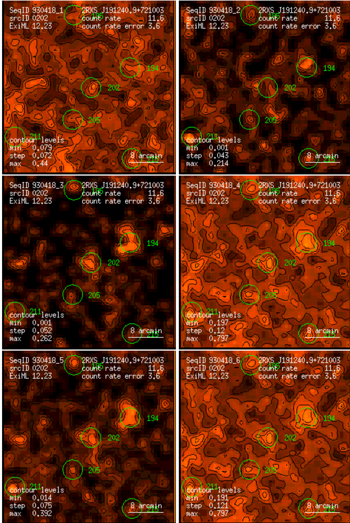
Figure 202: RASS 930418: detection 0202: band rate images, Gaussian filter: (1) PSPC channels 11 – 41, (2) 52 – 90, (3) 91 – 201, (4) 11 – 235, (5) 52 – 201, (6) 11 – 201. Broad band rates in counts/ks. Band rate contour levels in counts/ks/arcmin 2 .
