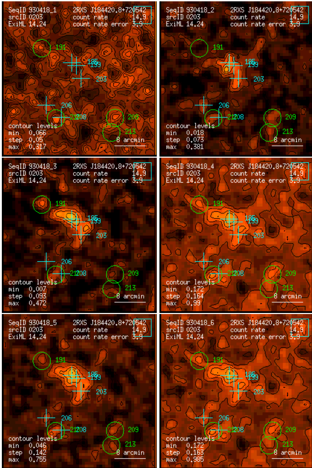
Figure 203: RASS 930418: detection 0203: band rate images, Gaussian filter: (1) PSPC channels 11 – 41, (2) 52 – 90, (3) 91 – 201, (4) 11 – 235, (5) 52 – 201, (6) 11 – 201. Broad band rates in counts/ks. Band rate contour levels in counts/ks/arcmin 2 .
