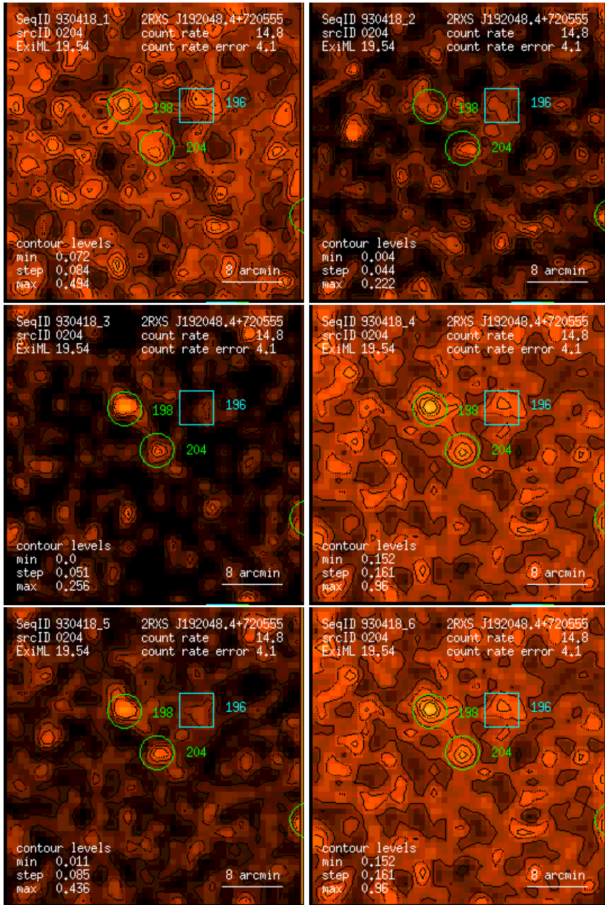
Figure 204: RASS 930418: detection 0204: band rate images, Gaussian filter: (1) PSPC channels 11 – 41, (2) 52 – 90, (3) 91 – 201, (4) 11 – 235, (5) 52 – 201, (6) 11 – 201. Broad band rates in counts/ks. Band rate contour levels in counts/ks/arcmin 2 .
