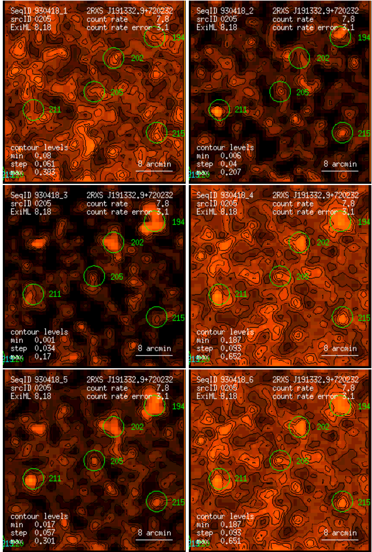
Figure 205: RASS 930418: detection 0205: band rate images, Gaussian filter: (1) PSPC channels 11 – 41, (2) 52 – 90, (3) 91 – 201, (4) 11 – 235, (5) 52 – 201, (6) 11 – 201. Broad band rates in counts/ks. Band rate contour levels in counts/ks/arcmin 2 .
