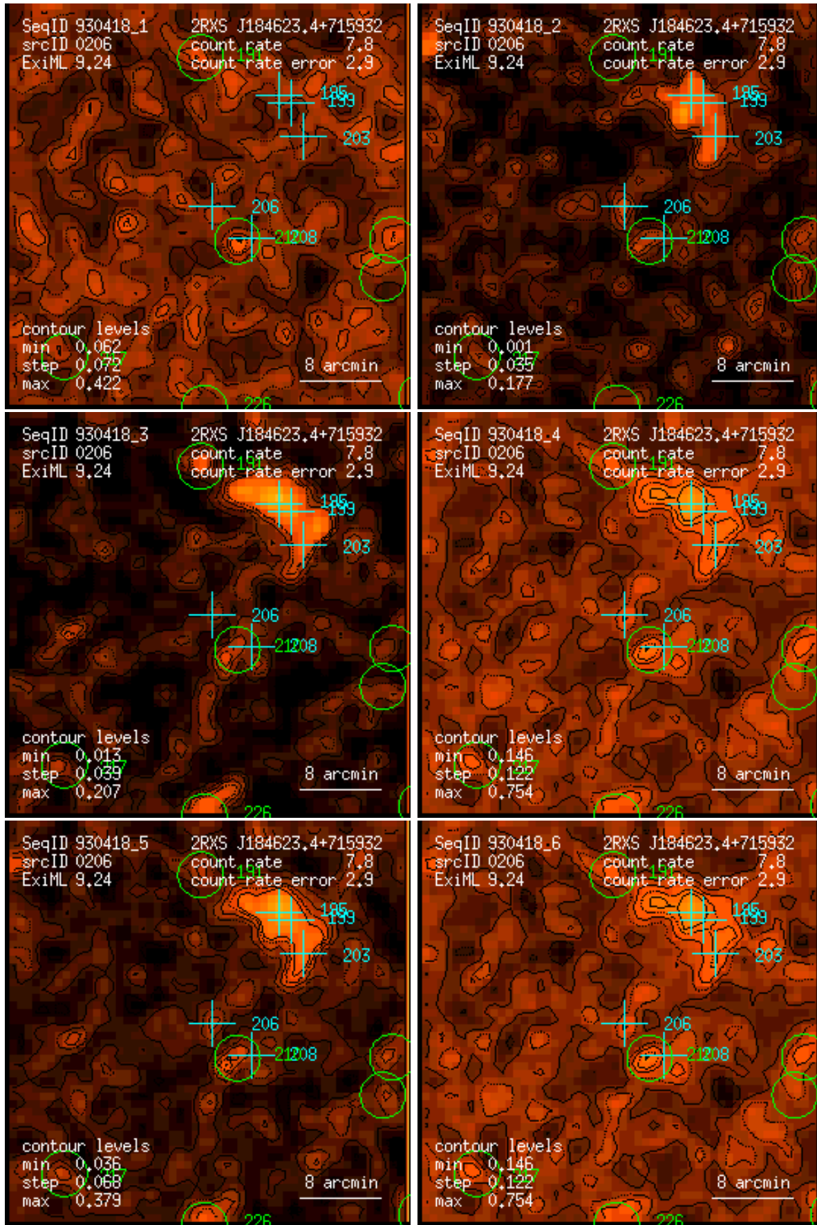
Figure 206: RASS 930418: detection 0206: band rate images, Gaussian filter: (1) PSPC channels 11 – 41, (2) 52 – 90, (3) 91 – 201, (4) 11 – 235, (5) 52 – 201, (6) 11 – 201. Broad band rates in counts/ks. Band rate contour levels in counts/ks/arcmin 2 .
