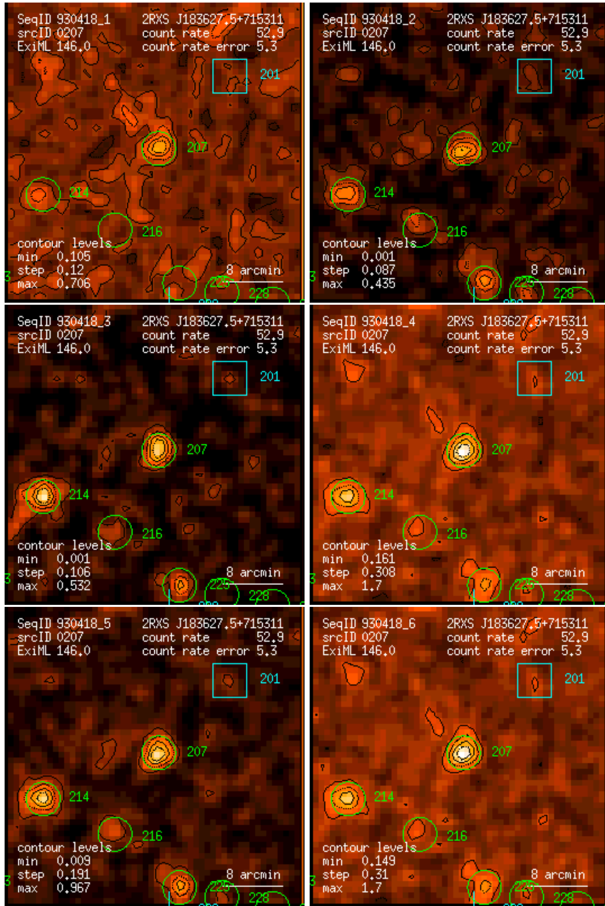
Figure 207: RASS 930418: detection 0207: band rate images, Gaussian filter: (1) PSPC channels 11 – 41, (2) 52 – 90, (3) 91 – 201, (4) 11 – 235, (5) 52 – 201, (6) 11 – 201. Broad band rates in counts/ks. Band rate contour levels in counts/ks/arcmin 2 .
