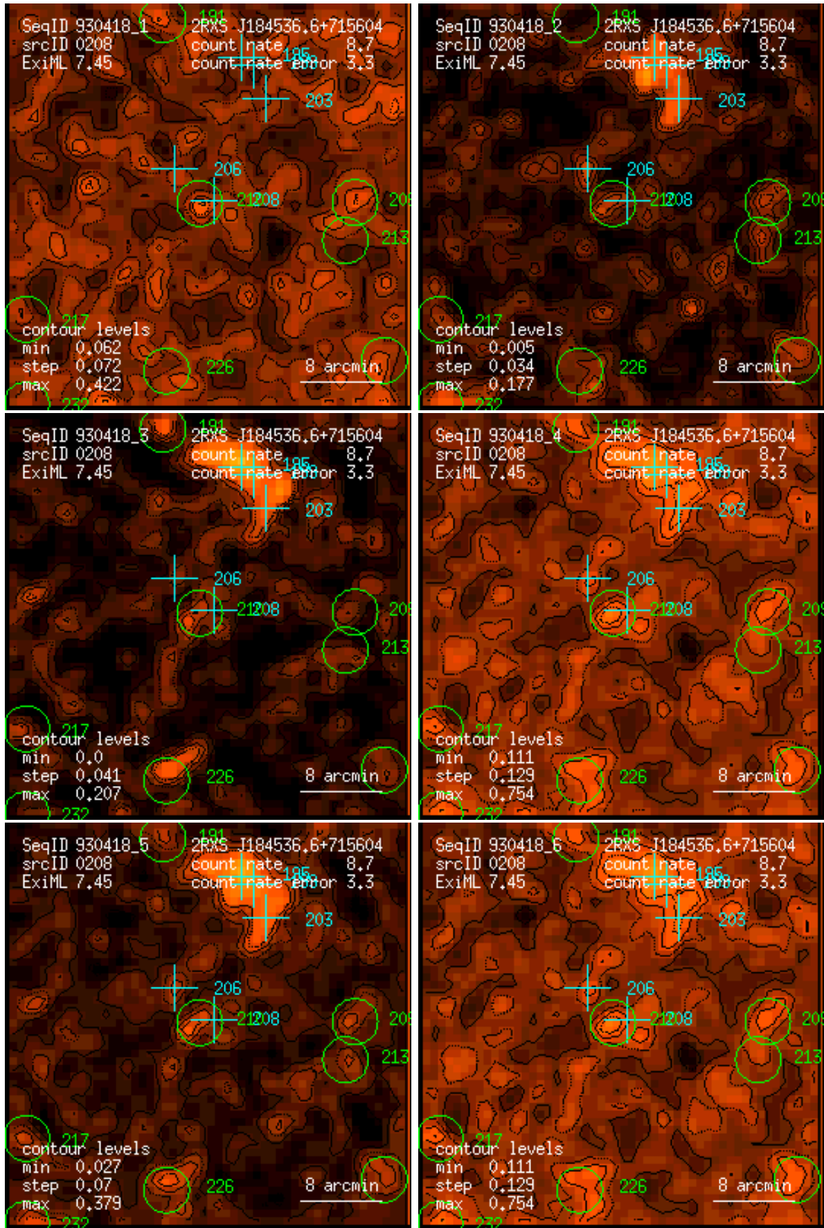
Figure 208: RASS 930418: detection 0208: band rate images, Gaussian filter: (1) PSPC channels 11 – 41, (2) 52 – 90, (3) 91 – 201, (4) 11 – 235, (5) 52 – 201, (6) 11 – 201. Broad band rates in counts/ks. Band rate contour levels in counts/ks/arcmin 2 .
