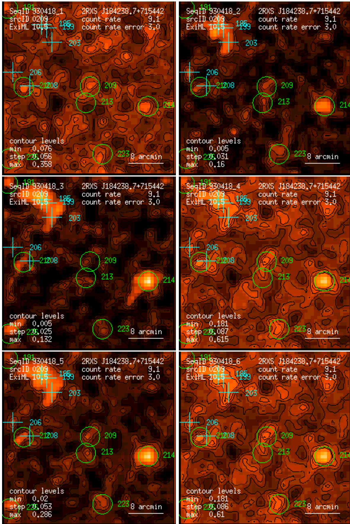
Figure 209: RASS 930418: detection 0209: band rate images, Gaussian filter: (1) PSPC channels 11 – 41, (2) 52 – 90, (3) 91 – 201, (4) 11 – 235, (5) 52 – 201, (6) 11 – 201. Broad band rates in counts/ks. Band rate contour levels in counts/ks/arcmin 2 .
