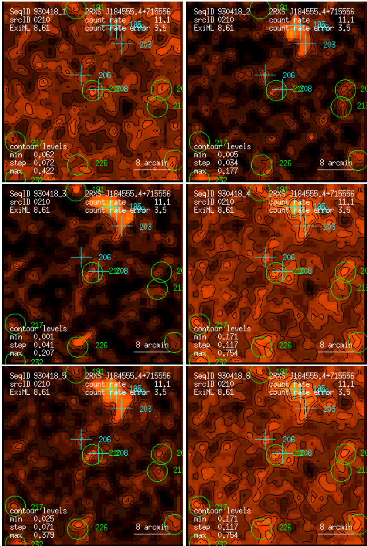
Figure 210: RASS 930418: detection 0210: band rate images, Gaussian filter: (1) PSPC channels 11 – 41, (2) 52 – 90, (3) 91 – 201, (4) 11 – 235, (5) 52 – 201, (6) 11 – 201. Broad band rates in counts/ks. Band rate contour levels in counts/ks/arcmin 2 .
