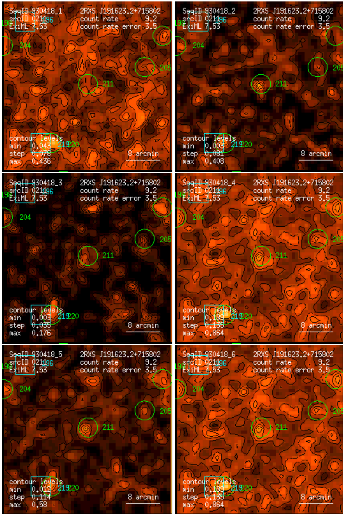
Figure 211: RASS 930418: detection 0211: band rate images, Gaussian filter: (1) PSPC channels 11 – 41, (2) 52 – 90, (3) 91 – 201, (4) 11 – 235, (5) 52 – 201, (6) 11 – 201. Broad band rates in counts/ks. Band rate contour levels in counts/ks/arcmin 2 .
