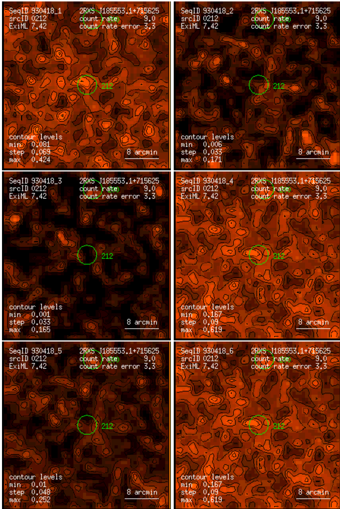
Figure 212: RASS 930418: detection 0212: band rate images, Gaussian filter: (1) PSPC channels 11 – 41, (2) 52 – 90, (3) 91 – 201, (4) 11 – 235, (5) 52 – 201, (6) 11 – 201. Broad band rates in counts/ks. Band rate contour levels in counts/ks/arcmin 2 .
