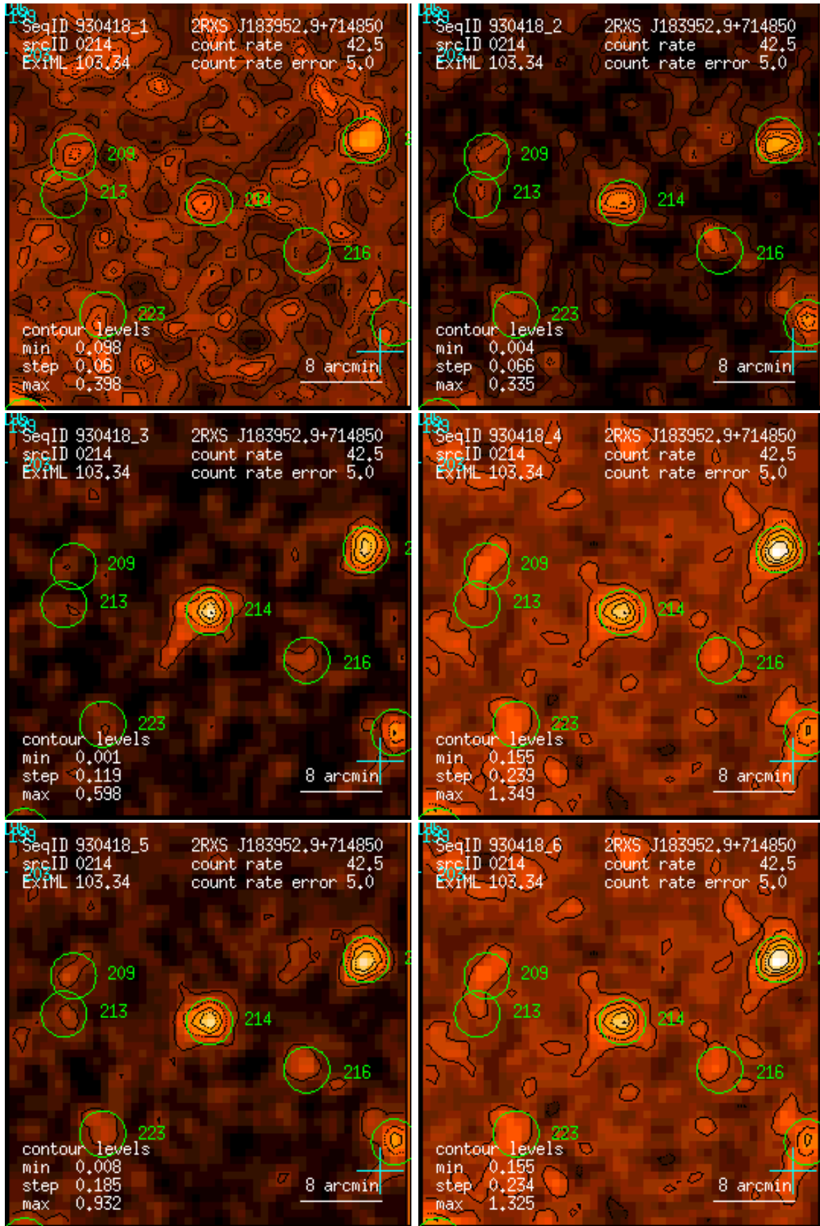
Figure 214: RASS 930418: detection 0214: band rate images, Gaussian filter: (1) PSPC channels 11 – 41, (2) 52 – 90, (3) 91 – 201, (4) 11 – 235, (5) 52 – 201, (6) 11 – 201. Broad band rates in counts/ks. Band rate contour levels in counts/ks/arcmin 2 .
