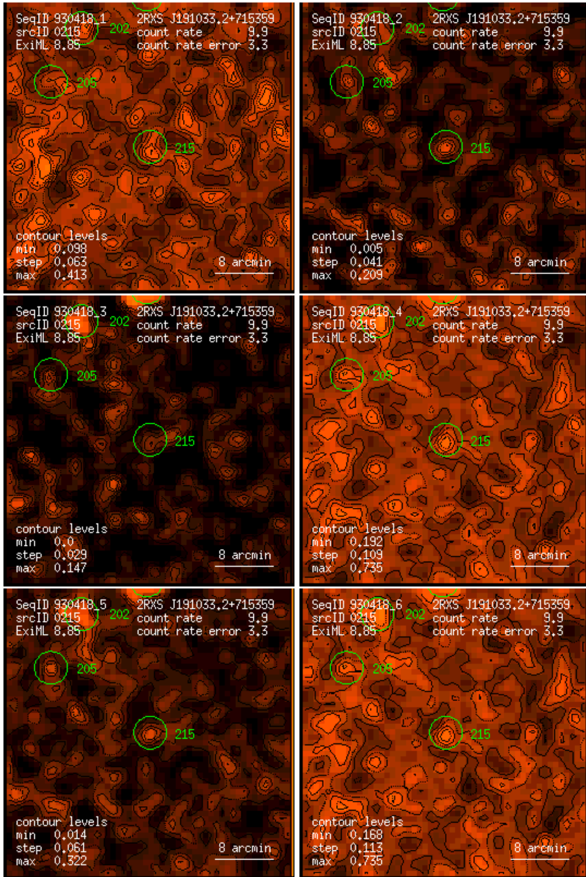
Figure 215: RASS 930418: detection 0215: band rate images, Gaussian filter: (1) PSPC channels 11 – 41, (2) 52 – 90, (3) 91 – 201, (4) 11 – 235, (5) 52 – 201, (6) 11 – 201. Broad band rates in counts/ks. Band rate contour levels in counts/ks/arcmin 2 .
