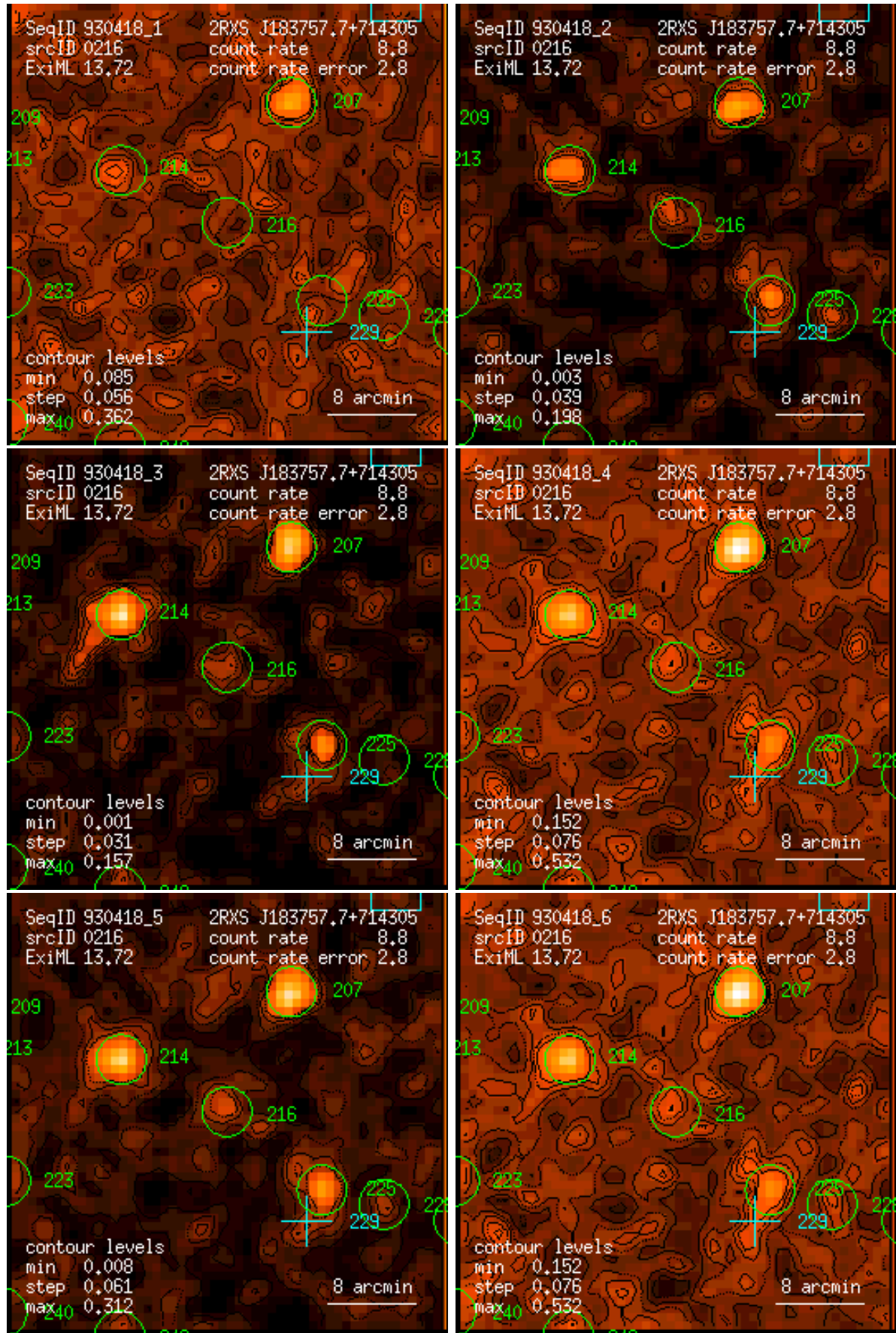
Figure 216: RASS 930418: detection 0216: band rate images, Gaussian filter: (1) PSPC channels 11 – 41, (2) 52 – 90, (3) 91 – 201, (4) 11 – 235, (5) 52 – 201, (6) 11 – 201. Broad band rates in counts/ks. Band rate contour levels in counts/ks/arcmin 2 .
