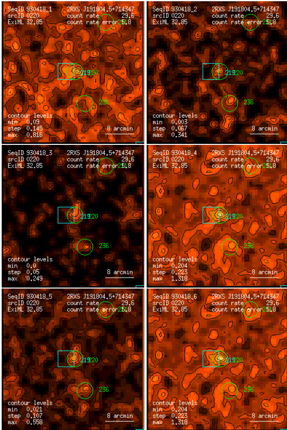
Figure 220: RASS 930418: detection 0220: band rate images, Gaussian filter: (1) PSPC channels 11 – 41, (2) 52 – 90, (3) 91 – 201, (4) 11 – 235, (5) 52 – 201, (6) 11 – 201. Broad band rates in counts/ks. Band rate contour levels in counts/ks/arcmin 2 .
