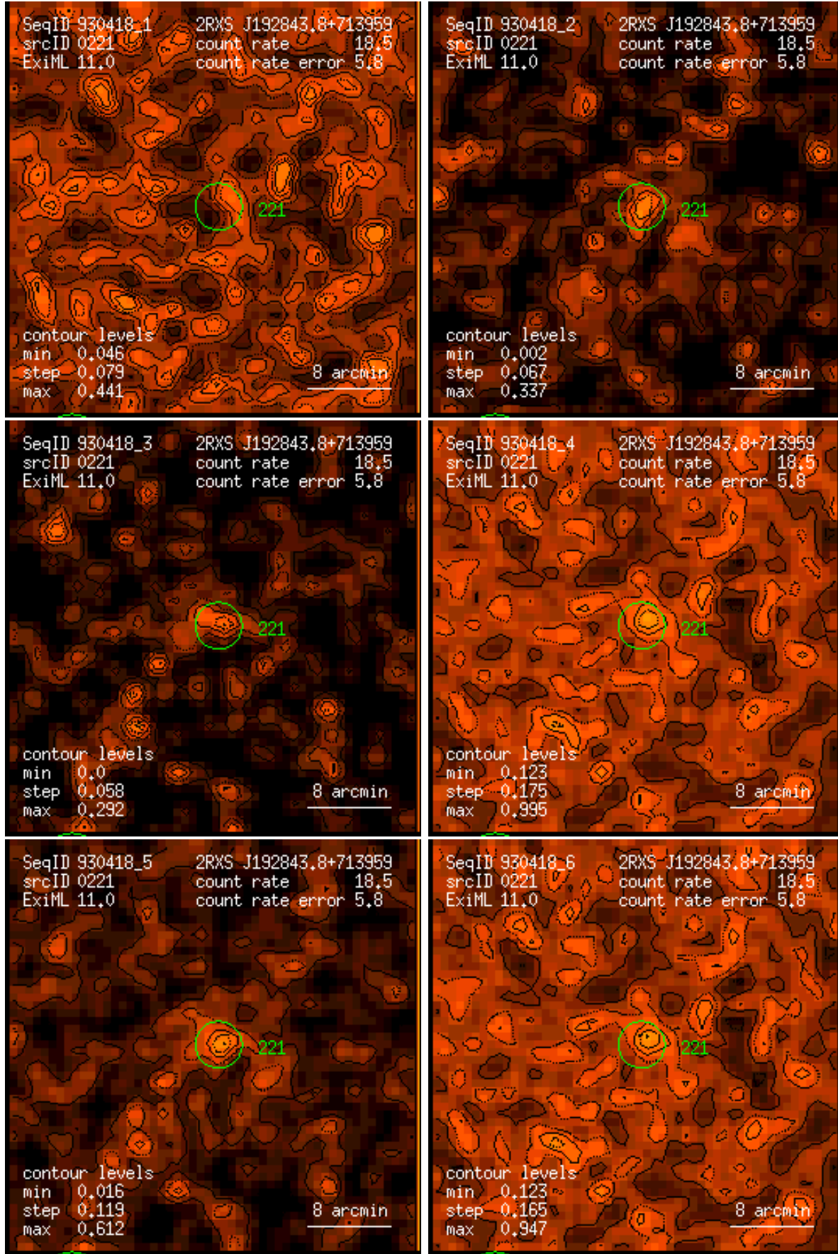
Figure 221: RASS 930418: detection 0221: band rate images, Gaussian filter: (1) PSPC channels 11 – 41, (2) 52 – 90, (3) 91 – 201, (4) 11 – 235, (5) 52 – 201, (6) 11 – 201. Broad band rates in counts/ks. Band rate contour levels in counts/ks/arcmin 2 .
