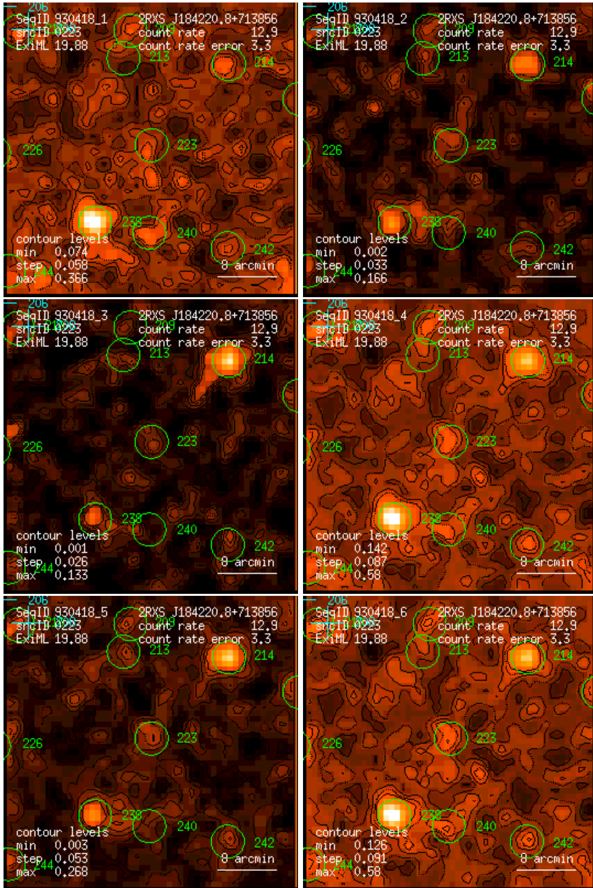
Figure 223: RASS 930418: detection 0223: band rate images, Gaussian filter: (1) PSPC channels 11 – 41, (2) 52 – 90, (3) 91 – 201, (4) 11 – 235, (5) 52 – 201, (6) 11 – 201. Broad band rates in counts/ks. Band rate contour levels in counts/ks/arcmin 2 .
