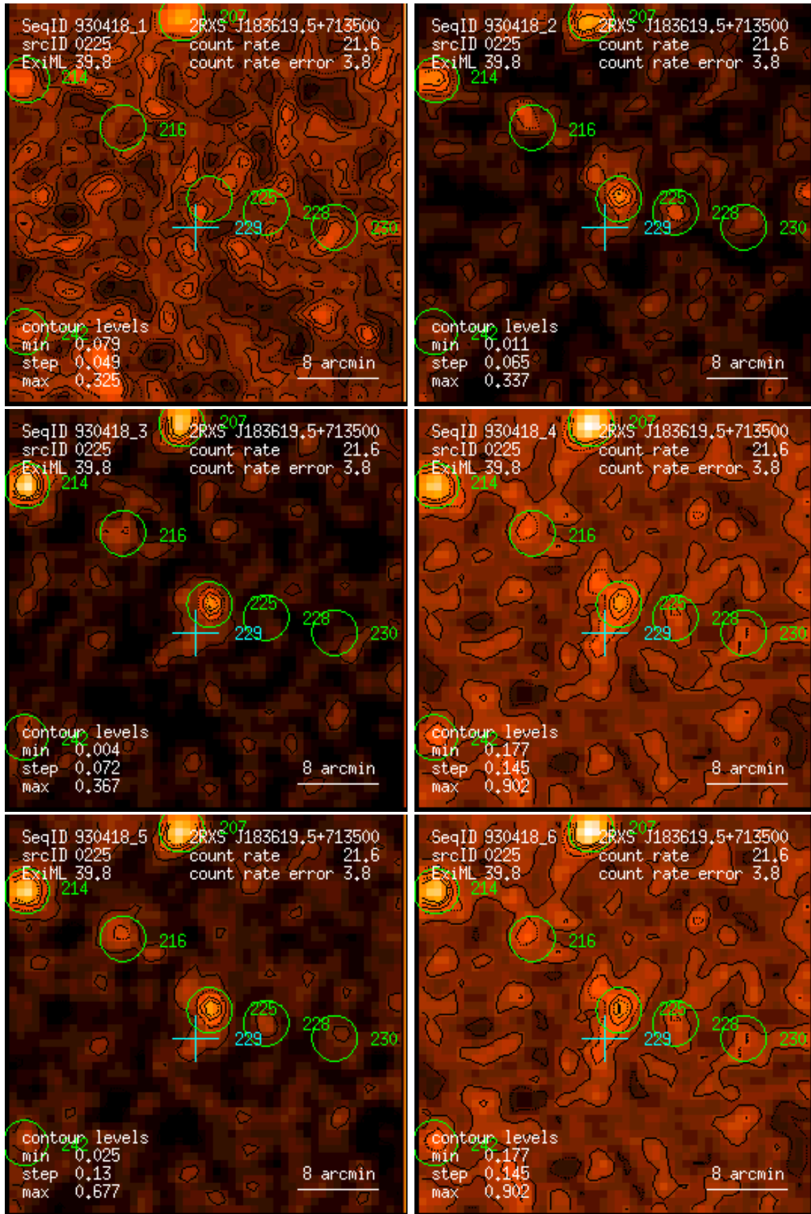
Figure 225: RASS 930418: detection 0225: band rate images, Gaussian filter: (1) PSPC channels 11 – 41, (2) 52 – 90, (3) 91 – 201, (4) 11 – 235, (5) 52 – 201, (6) 11 – 201. Broad band rates in counts/ks. Band rate contour levels in counts/ks/arcmin 2 .
