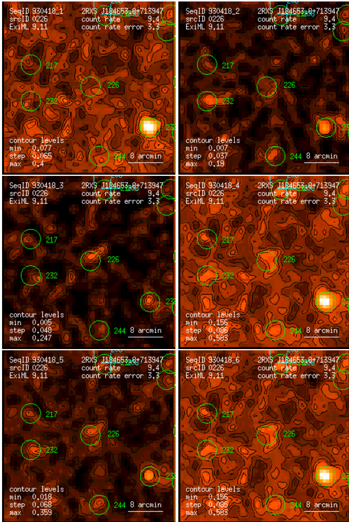
Figure 226: RASS 930418: detection 0226: band rate images, Gaussian filter: (1) PSPC channels 11 – 41, (2) 52 – 90, (3) 91 – 201, (4) 11 – 235, (5) 52 – 201, (6) 11 – 201. Broad band rates in counts/ks. Band rate contour levels in counts/ks/arcmin 2 .
