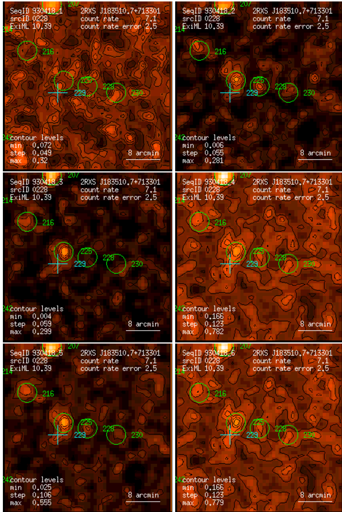
Figure 228: RASS 930418: detection 0228: band rate images, Gaussian filter: (1) PSPC channels 11 – 41, (2) 52 – 90, (3) 91 – 201, (4) 11 – 235, (5) 52 – 201, (6) 11 – 201. Broad band rates in counts/ks. Band rate contour levels in counts/ks/arcmin 2 .
