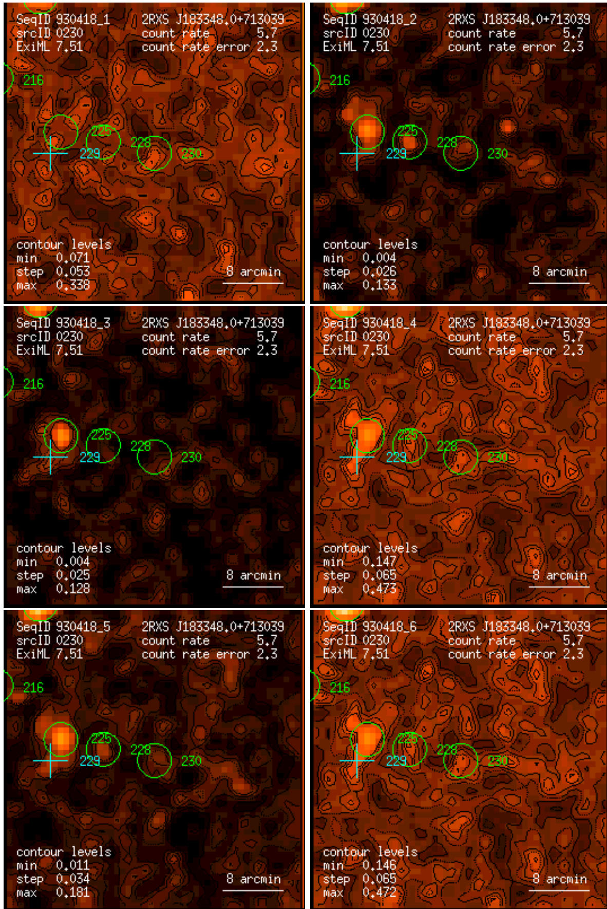
Figure 230: RASS 930418: detection 0230: band rate images, Gaussian filter: (1) PSPC channels 11 – 41, (2) 52 – 90, (3) 91 – 201, (4) 11 – 235, (5) 52 – 201, (6) 11 – 201. Broad band rates in counts/ks. Band rate contour levels in counts/ks/arcmin 2 .
