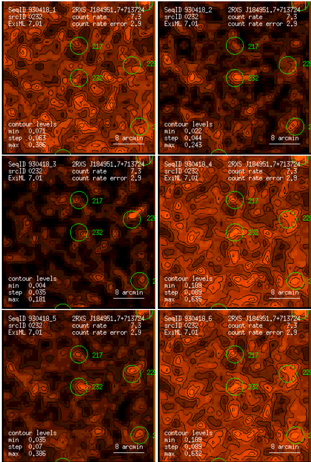
Figure 232: RASS 930418: detection 0232: band rate images, Gaussian filter: (1) PSPC channels 11 – 41, (2) 52 – 90, (3) 91 – 201, (4) 11 – 235, (5) 52 – 201, (6) 11 – 201. Broad band rates in counts/ks. Band rate contour levels in counts/ks/arcmin 2 .
