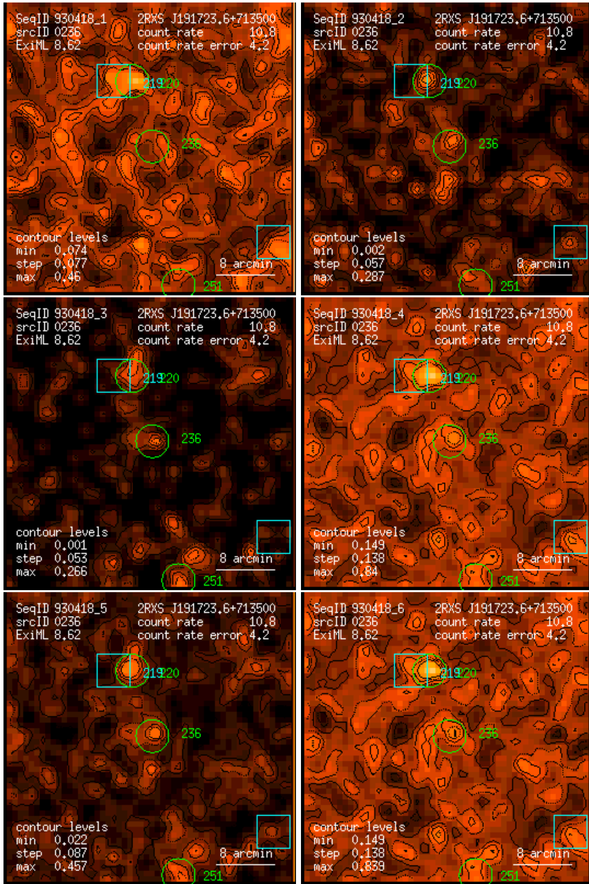
Figure 236: RASS 930418: detection 0236: band rate images, Gaussian filter: (1) PSPC channels 11 – 41, (2) 52 – 90, (3) 91 – 201, (4) 11 – 235, (5) 52 – 201, (6) 11 – 201. Broad band rates in counts/ks. Band rate contour levels in counts/ks/arcmin 2 .
