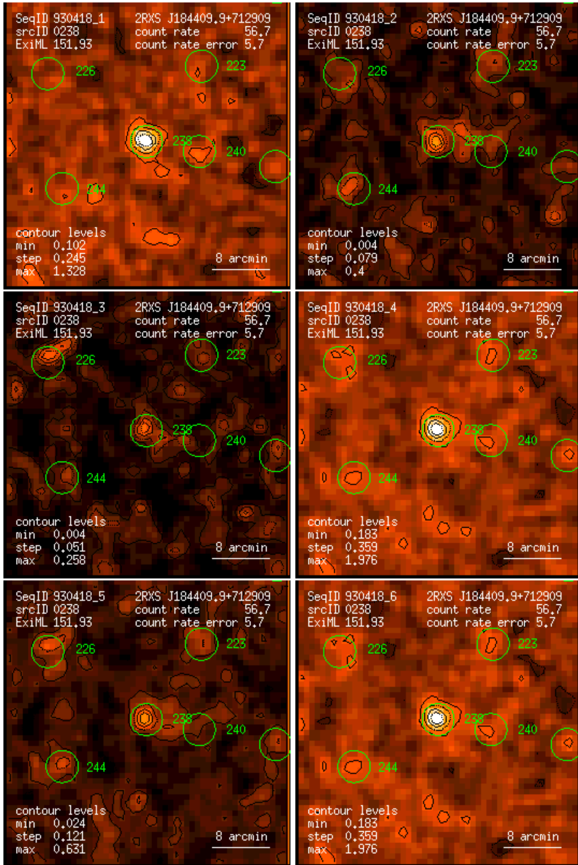
Figure 238: RASS 930418: detection 0238: band rate images, Gaussian filter: (1) PSPC channels 11 – 41, (2) 52 – 90, (3) 91 – 201, (4) 11 – 235, (5) 52 – 201, (6) 11 – 201. Broad band rates in counts/ks. Band rate contour levels in counts/ks/arcmin 2 .
