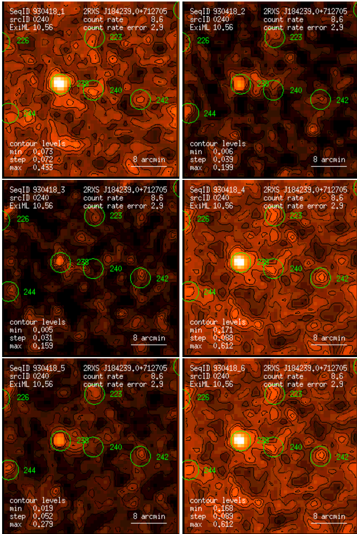
Figure 240: RASS 930418: detection 0240: band rate images, Gaussian filter: (1) PSPC channels 11 – 41, (2) 52 – 90, (3) 91 – 201, (4) 11 – 235, (5) 52 – 201, (6) 11 – 201. Broad band rates in counts/ks. Band rate contour levels in counts/ks/arcmin 2 .
