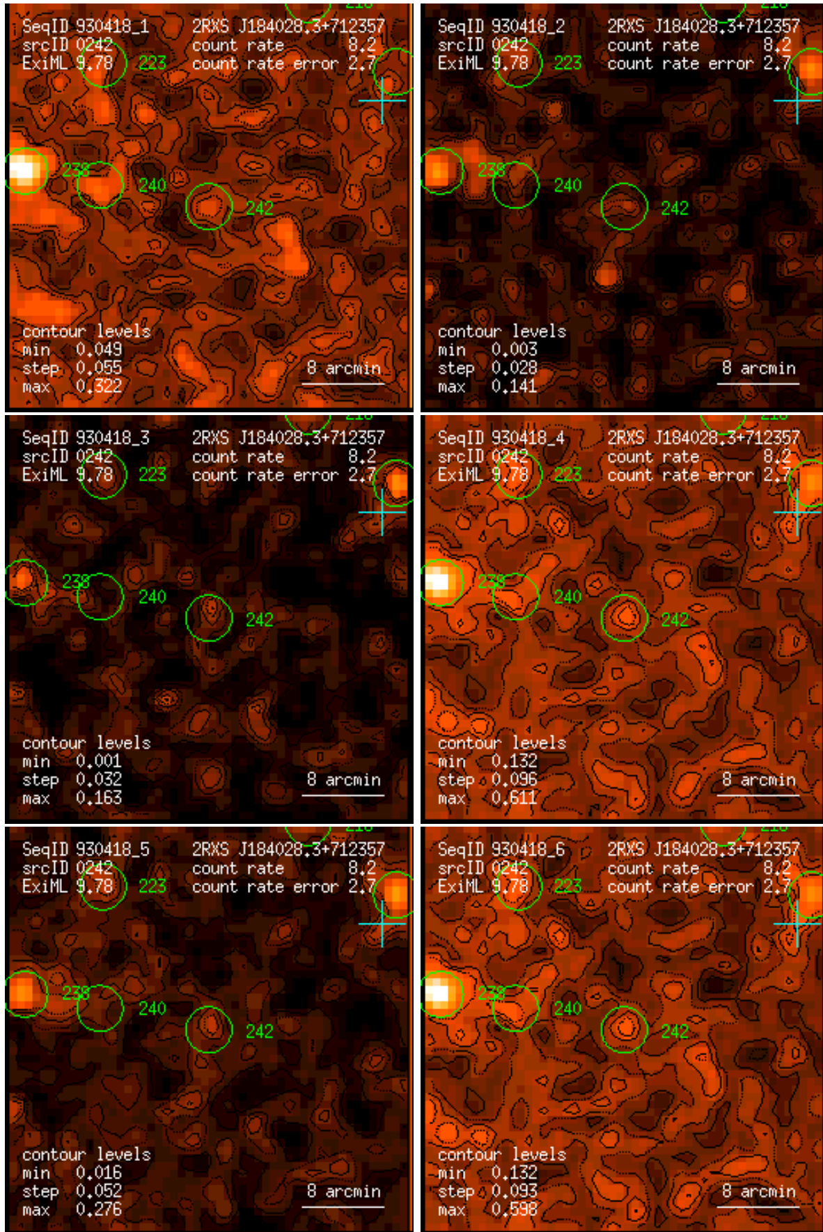
Figure 242: RASS 930418: detection 0242: band rate images, Gaussian filter: (1) PSPC channels 11 – 41, (2) 52 – 90, (3) 91 – 201, (4) 11 – 235, (5) 52 – 201, (6) 11 – 201. Broad band rates in counts/ks. Band rate contour levels in counts/ks/arcmin 2 .
