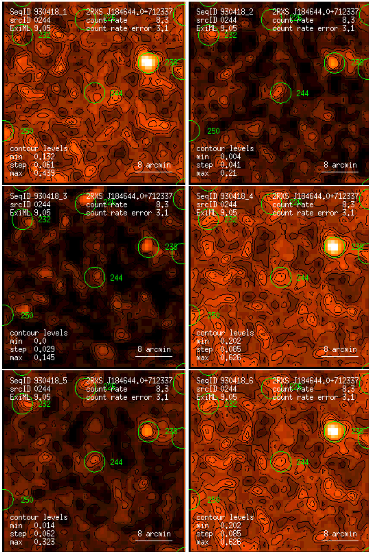
Figure 244: RASS 930418: detection 0244: band rate images, Gaussian filter: (1) PSPC channels 11 – 41, (2) 52 – 90, (3) 91 – 201, (4) 11 – 235, (5) 52 – 201, (6) 11 – 201. Broad band rates in counts/ks. Band rate contour levels in counts/ks/arcmin 2 .
