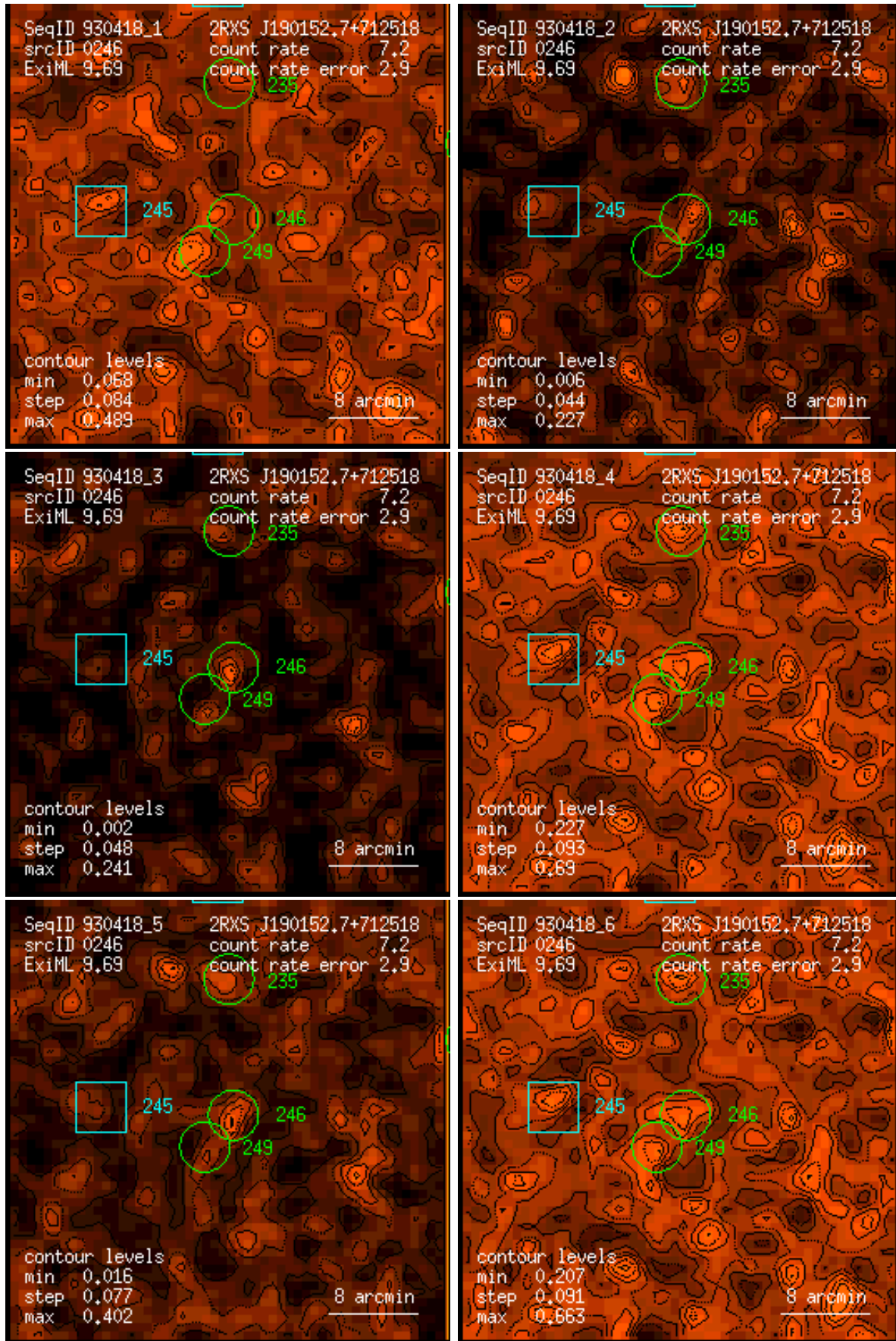
Figure 246: RASS 930418: detection 0246: band rate images, Gaussian filter: (1) PSPC channels 11 – 41, (2) 52 – 90, (3) 91 – 201, (4) 11 – 235, (5) 52 – 201, (6) 11 – 201. Broad band rates in counts/ks. Band rate contour levels in counts/ks/arcmin 2 .
