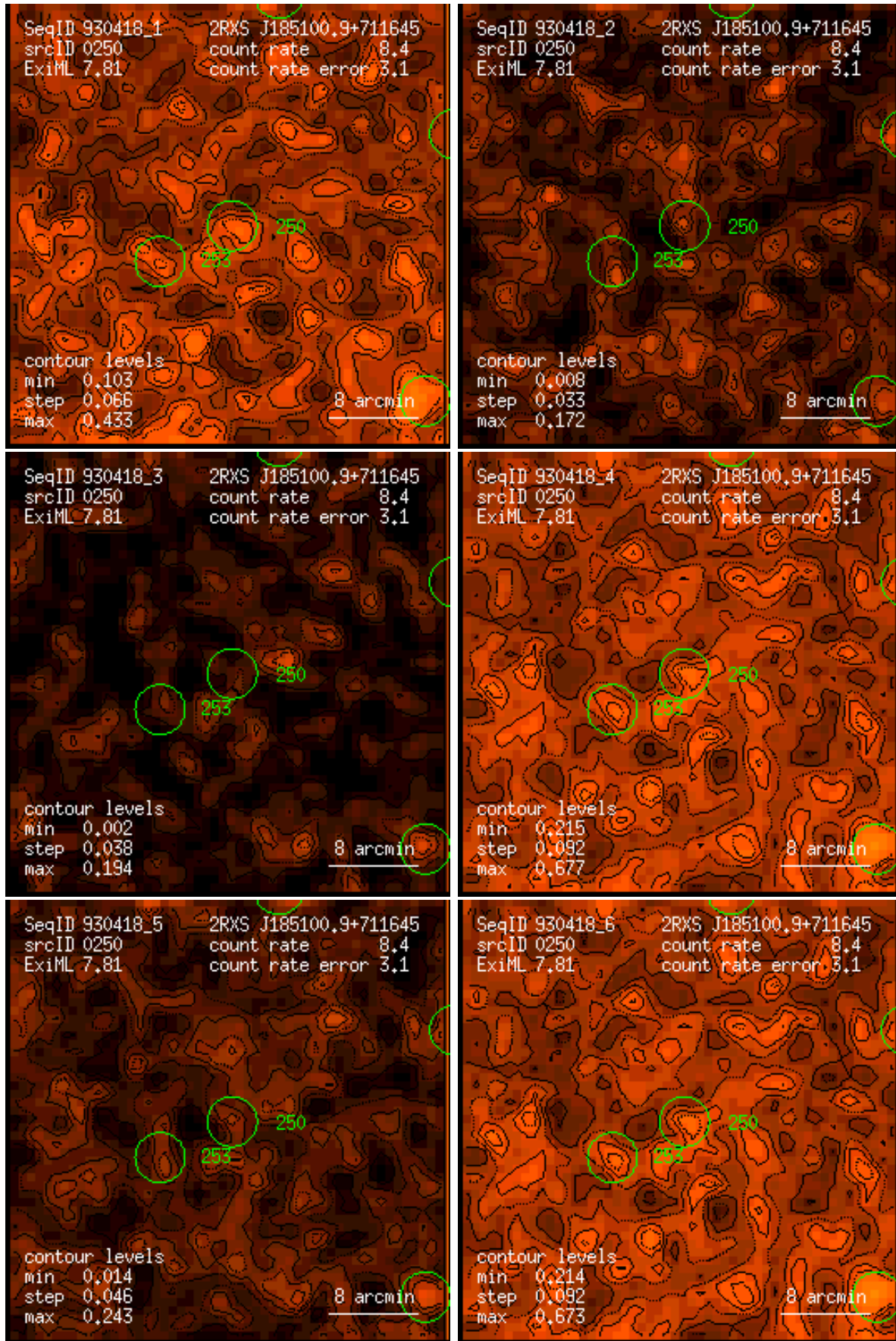
Figure 250: RASS 930418: detection 0250: band rate images, Gaussian filter: (1) PSPC channels 11 – 41, (2) 52 – 90, (3) 91 – 201, (4) 11 – 235, (5) 52 – 201, (6) 11 – 201. Broad band rates in counts/ks. Band rate contour levels in counts/ks/arcmin 2 .
