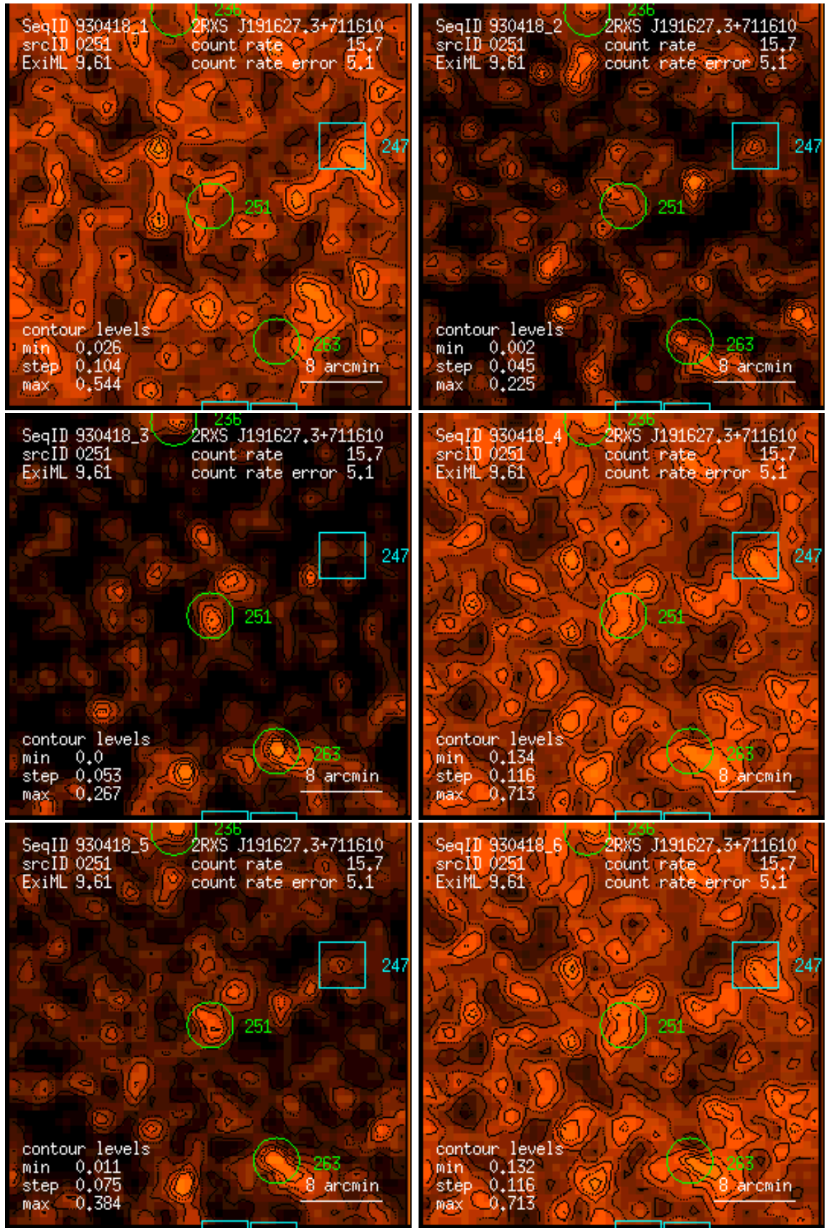
Figure 251: RASS 930418: detection 0251: band rate images, Gaussian filter: (1) PSPC channels 11 – 41, (2) 52 – 90, (3) 91 – 201, (4) 11 – 235, (5) 52 – 201, (6) 11 – 201. Broad band rates in counts/ks. Band rate contour levels in counts/ks/arcmin 2 .
