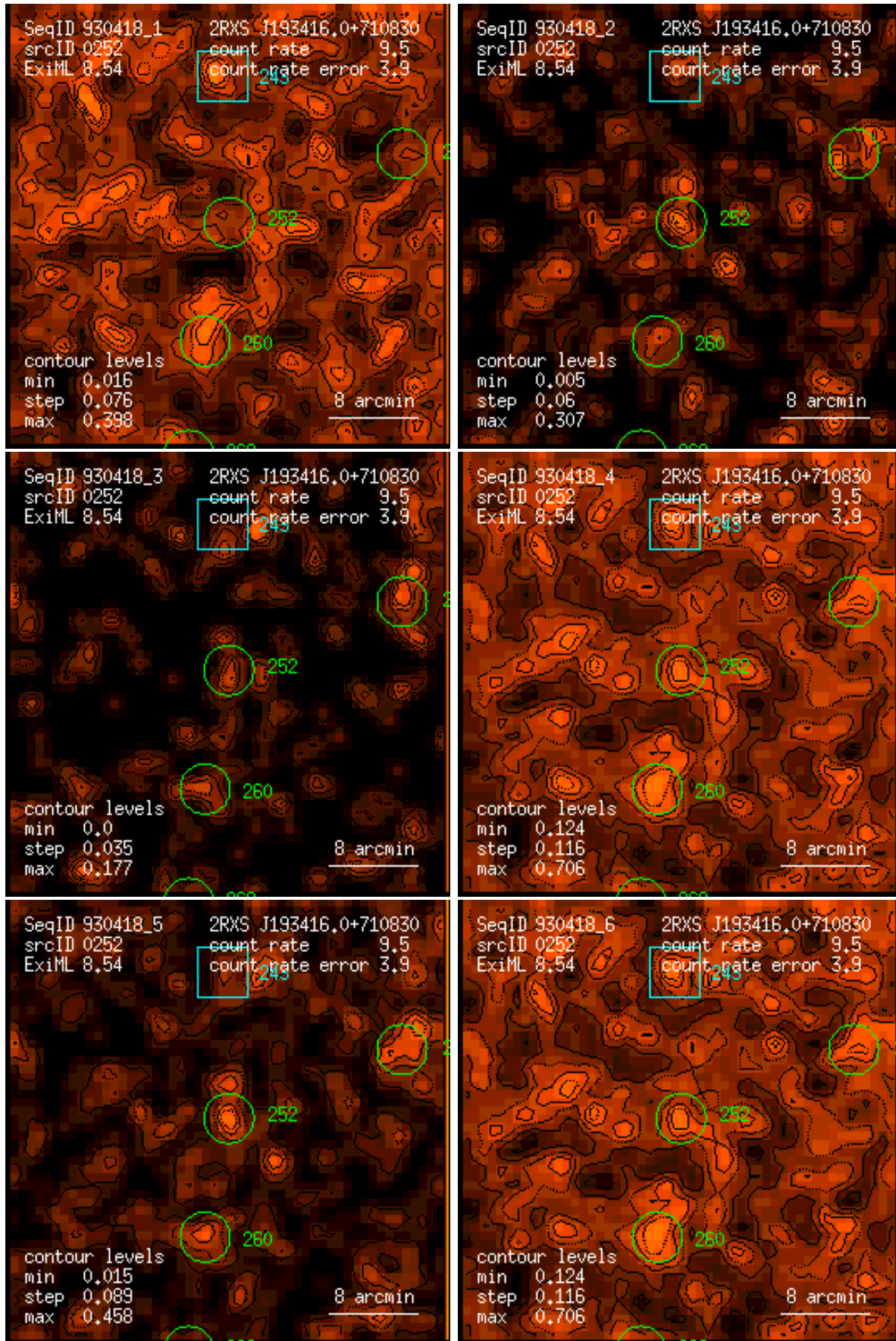
Figure 252: RASS 930418: detection 0252: band rate images, Gaussian filter: (1) PSPC channels 11 – 41, (2) 52 – 90, (3) 91 – 201, (4) 11 – 235, (5) 52 – 201, (6) 11 – 201. Broad band rates in counts/ks. Band rate contour levels in counts/ks/arcmin 2 .
