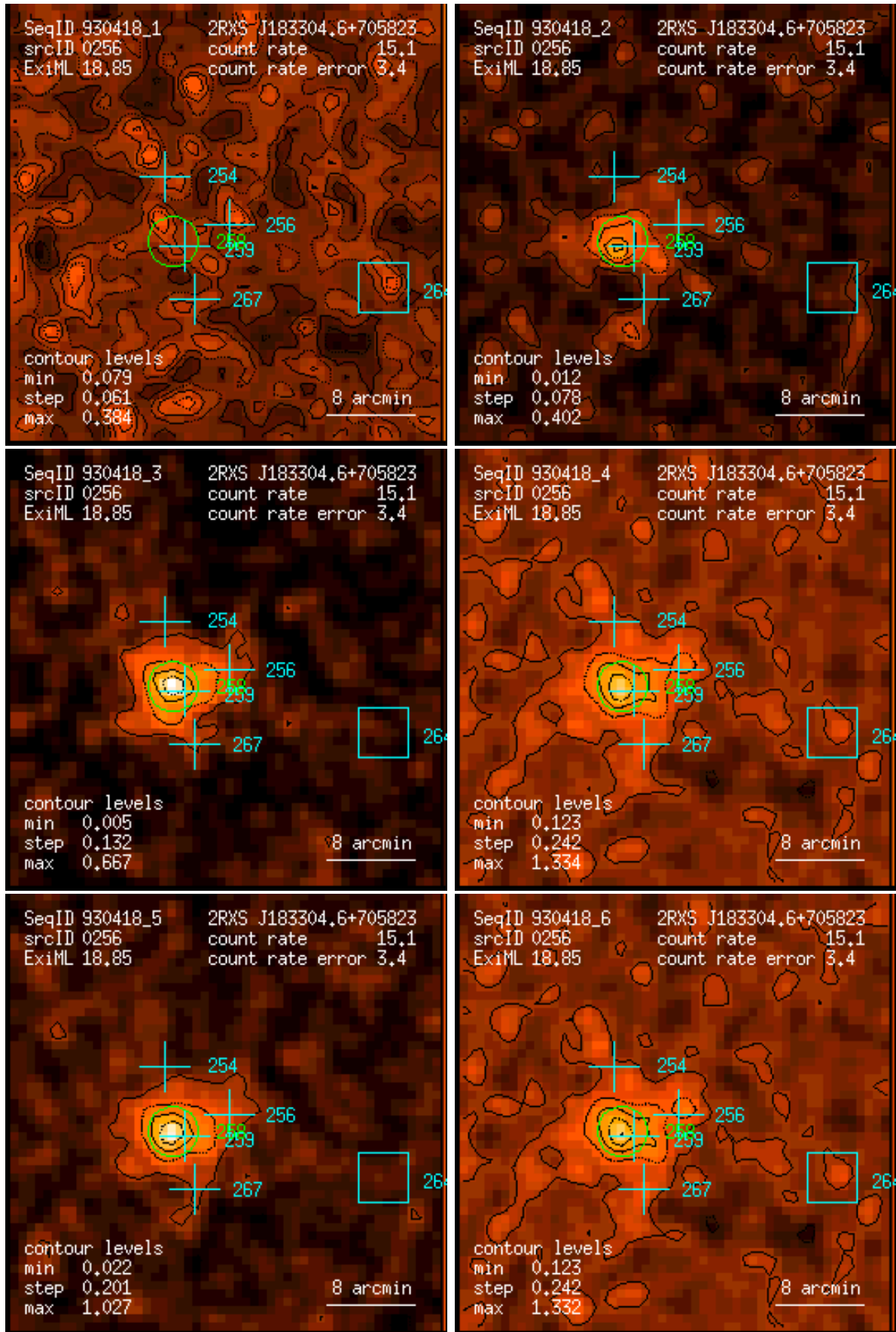
Figure 256: RASS 930418: detection 0256: band rate images, Gaussian filter: (1) PSPC channels 11 – 41, (2) 52 – 90, (3) 91 – 201, (4) 11 – 235, (5) 52 – 201, (6) 11 – 201. Broad band rates in counts/ks. Band rate contour levels in counts/ks/arcmin 2 .
