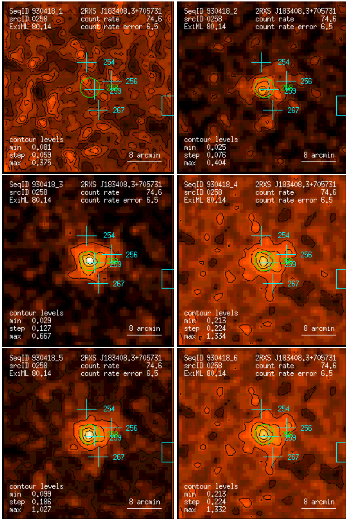
Figure 258: RASS 930418: detection 0258: band rate images, Gaussian filter: (1) PSPC channels 11 – 41, (2) 52 – 90, (3) 91 – 201, (4) 11 – 235, (5) 52 – 201, (6) 11 – 201. Broad band rates in counts/ks. Band rate contour levels in counts/ks/arcmin 2 .
