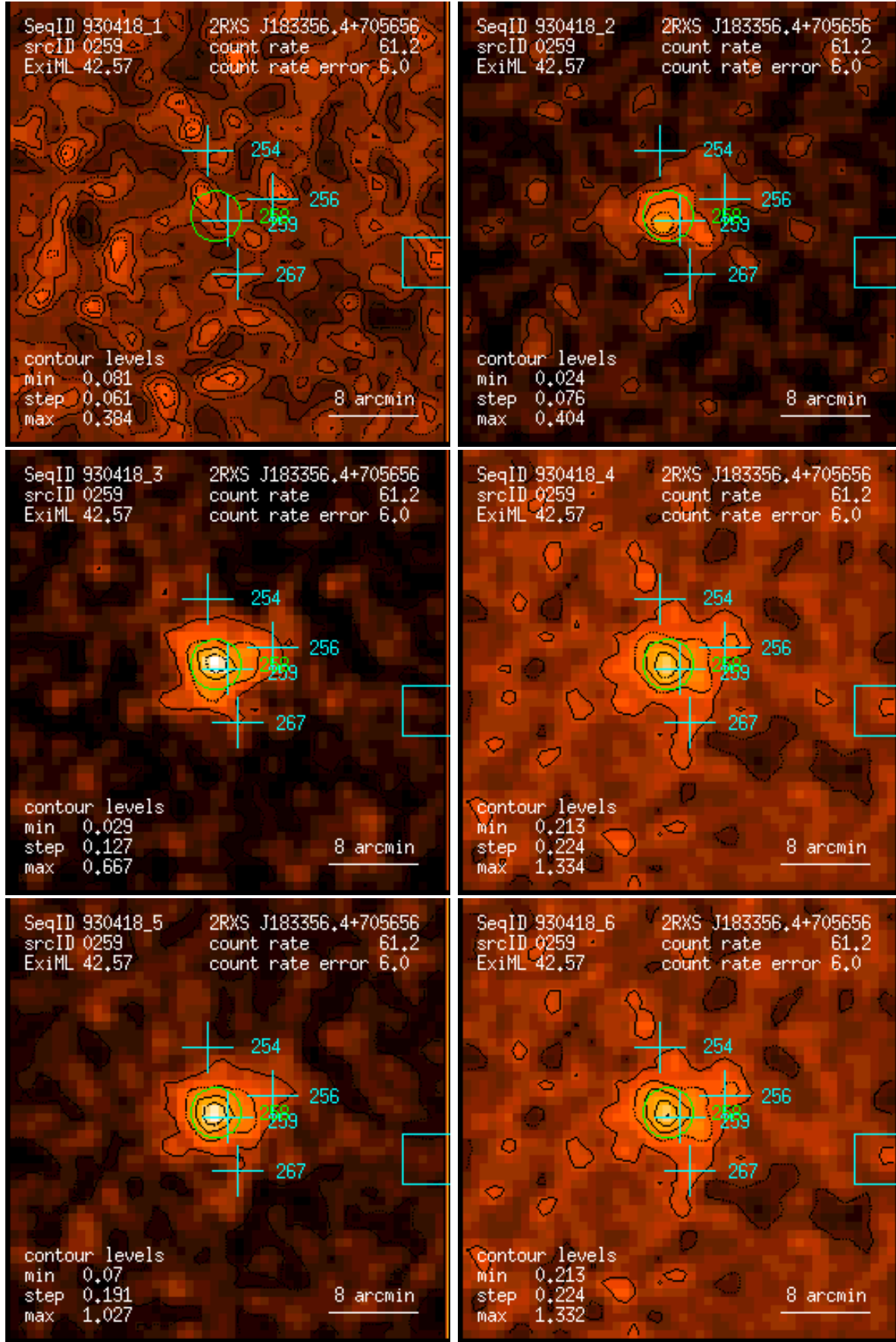
Figure 259: RASS 930418: detection 0259: band rate images, Gaussian filter: (1) PSPC channels 11 – 41, (2) 52 – 90, (3) 91 – 201, (4) 11 – 235, (5) 52 – 201, (6) 11 – 201. Broad band rates in counts/ks. Band rate contour levels in counts/ks/arcmin 2 .
