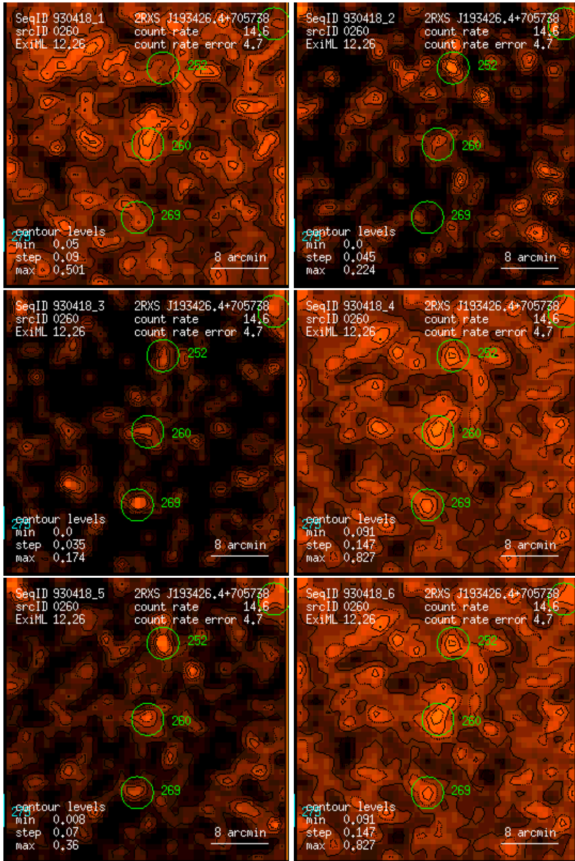
Figure 260: RASS 930418: detection 0260: band rate images, Gaussian filter: (1) PSPC channels 11 – 41, (2) 52 – 90, (3) 91 – 201, (4) 11 – 235, (5) 52 – 201, (6) 11 – 201. Broad band rates in counts/ks. Band rate contour levels in counts/ks/arcmin 2 .
